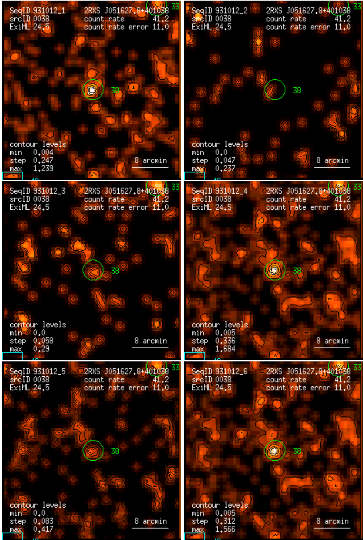
Figure 38: RASS 931012: detection 0038: band rate images, Gaussian filter: (1) PSPC channels 11 – 41, (2) 52 – 90, (3) 91 – 201, (4) 11 – 235, (5) 52 – 201, (6) 11 – 201. Broad band rates in counts/ks. Band rate contour levels in counts/ks/arcmin 2 .
