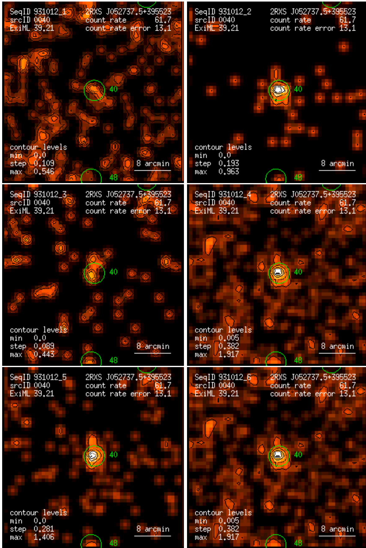
Figure 40: RASS 931012: detection 0040: band rate images, Gaussian filter: (1) PSPC channels 11 – 41, (2) 52 – 90, (3) 91 – 201, (4) 11 – 235, (5) 52 – 201, (6) 11 – 201. Broad band rates in counts/ks. Band rate contour levels in counts/ks/arcmin 2 .
