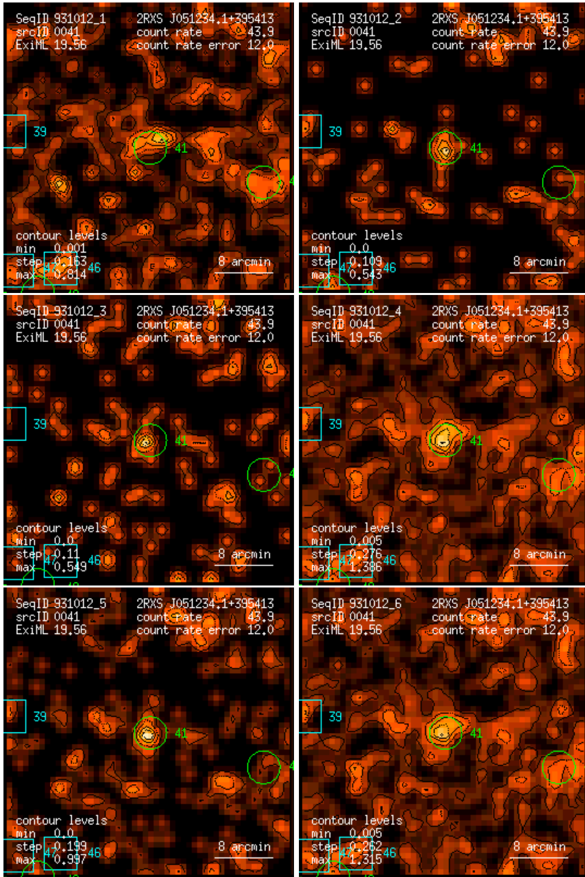
Figure 41: RASS 931012: detection 0041: band rate images, Gaussian filter: (1) PSPC channels 11 – 41, (2) 52 – 90, (3) 91 – 201, (4) 11 – 235, (5) 52 – 201, (6) 11 – 201. Broad band rates in counts/ks. Band rate contour levels in counts/ks/arcmin 2 .
