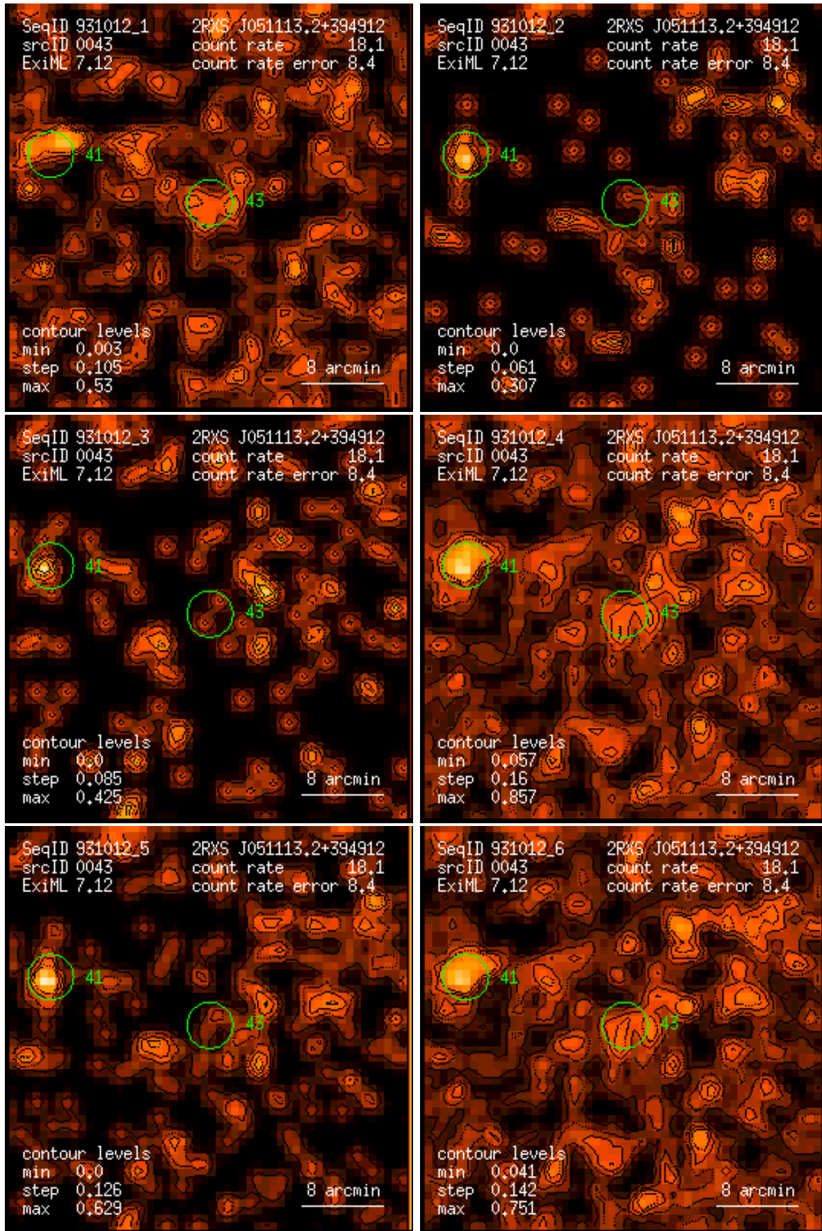
Figure 43: RASS 931012: detection 0043: band rate images, Gaussian filter: (1) PSPC channels 11 – 41, (2) 52 – 90, (3) 91 – 201, (4) 11 – 235, (5) 52 – 201, (6) 11 – 201. Broad band rates in counts/ks. Band rate contour levels in counts/ks/arcmin 2 .
