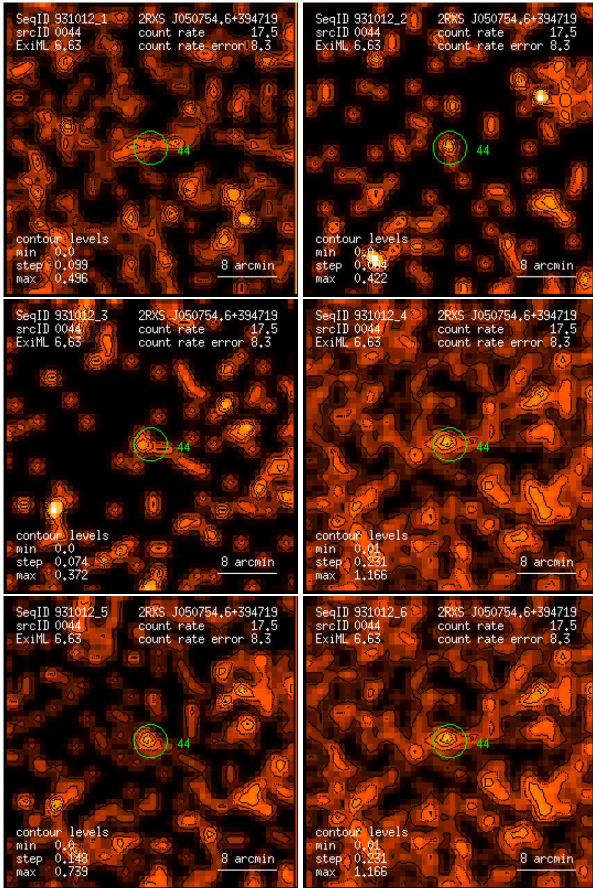
Figure 44: RASS 931012: detection 0044: band rate images, Gaussian filter: (1) PSPC channels 11 – 41, (2) 52 – 90, (3) 91 – 201, (4) 11 – 235, (5) 52 – 201, (6) 11 – 201. Broad band rates in counts/ks. Band rate contour levels in counts/ks/arcmin 2 .
