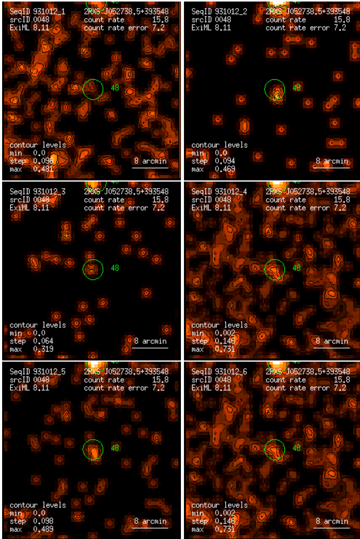
Figure 48: RASS 931012: detection 0048: band rate images, Gaussian filter: (1) PSPC channels 11 – 41, (2) 52 – 90, (3) 91 – 201, (4) 11 – 235, (5) 52 – 201, (6) 11 – 201. Broad band rates in counts/ks. Band rate contour levels in counts/ks/arcmin 2 .
