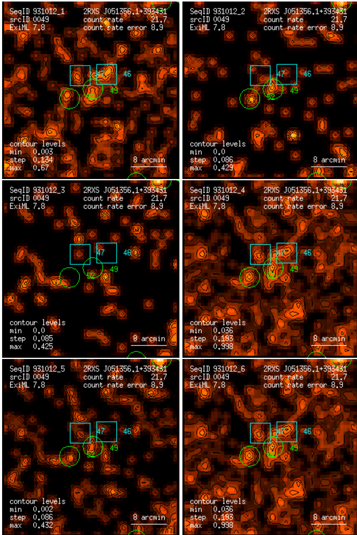
Figure 49: RASS 931012: detection 0049: band rate images, Gaussian filter: (1) PSPC channels 11 – 41, (2) 52 – 90, (3) 91 – 201, (4) 11 – 235, (5) 52 – 201, (6) 11 – 201. Broad band rates in counts/ks. Band rate contour levels in counts/ks/arcmin 2 .
