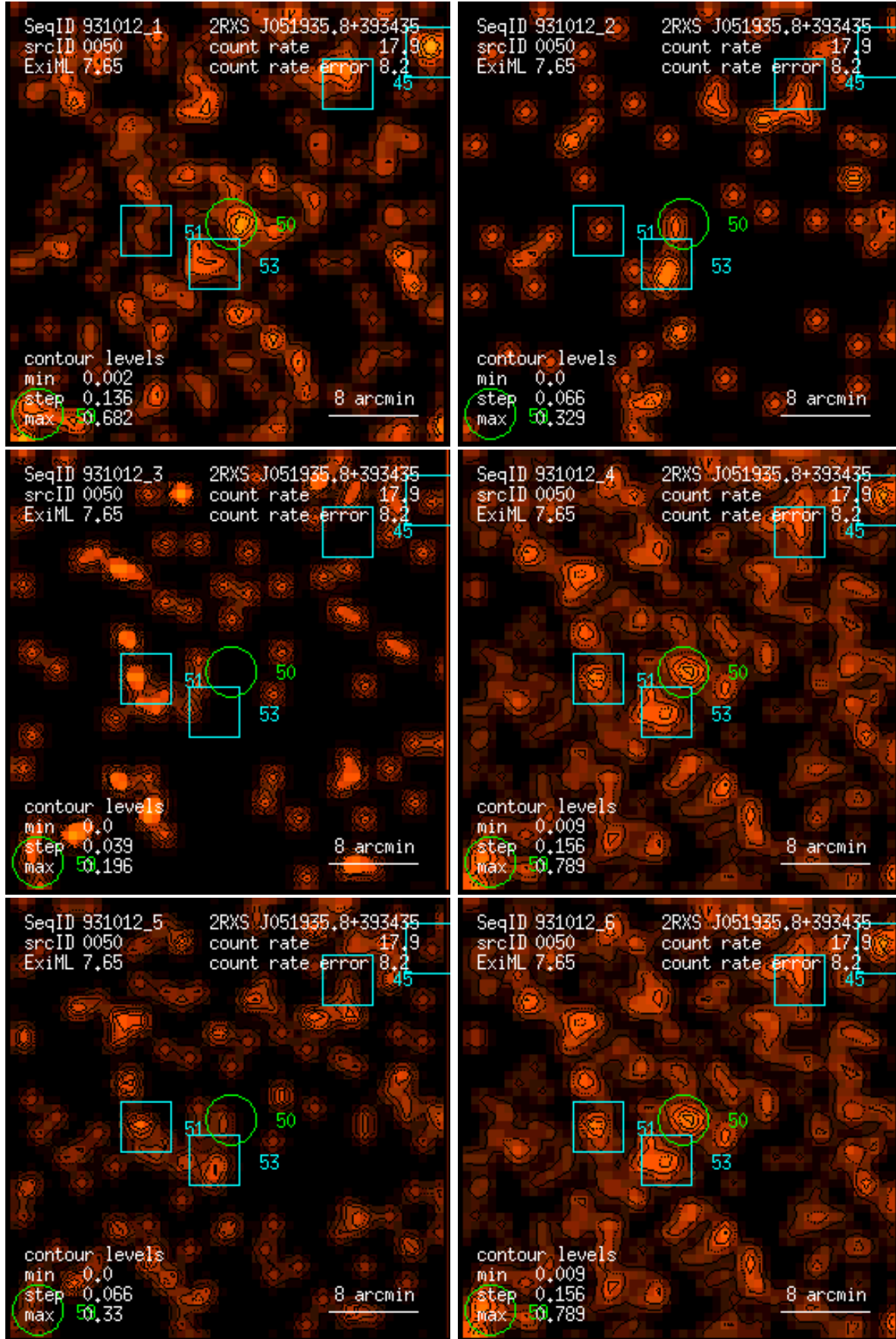
Figure 50: RASS 931012: detection 0050: band rate images, Gaussian filter: (1) PSPC channels 11 – 41, (2) 52 – 90, (3) 91 – 201, (4) 11 – 235, (5) 52 – 201, (6) 11 – 201. Broad band rates in counts/ks. Band rate contour levels in counts/ks/arcmin 2 .
