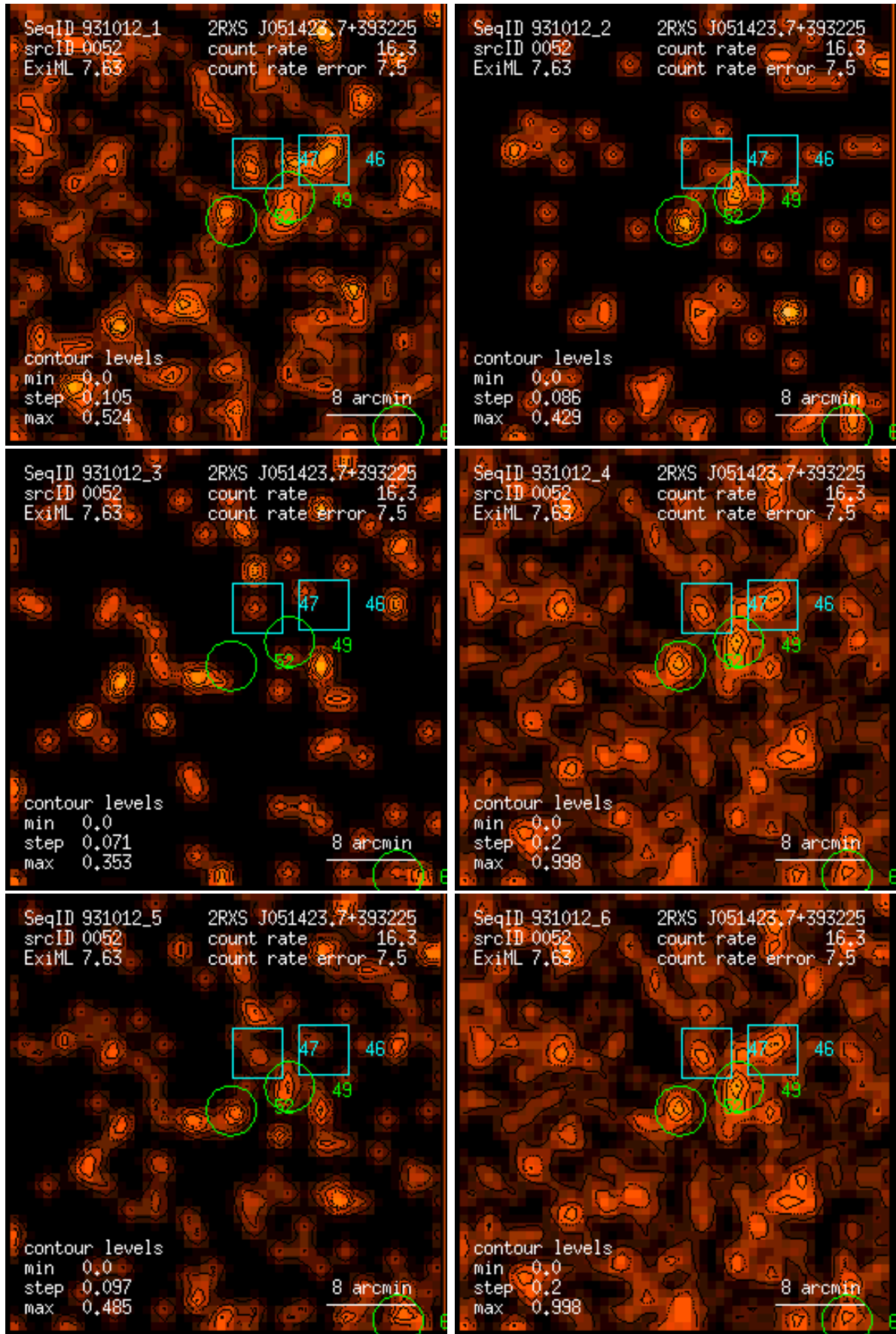
Figure 52: RASS 931012: detection 0052: band rate images, Gaussian filter: (1) PSPC channels 11 – 41, (2) 52 – 90, (3) 91 – 201, (4) 11 – 235, (5) 52 – 201, (6) 11 – 201. Broad band rates in counts/ks. Band rate contour levels in counts/ks/arcmin 2 .
