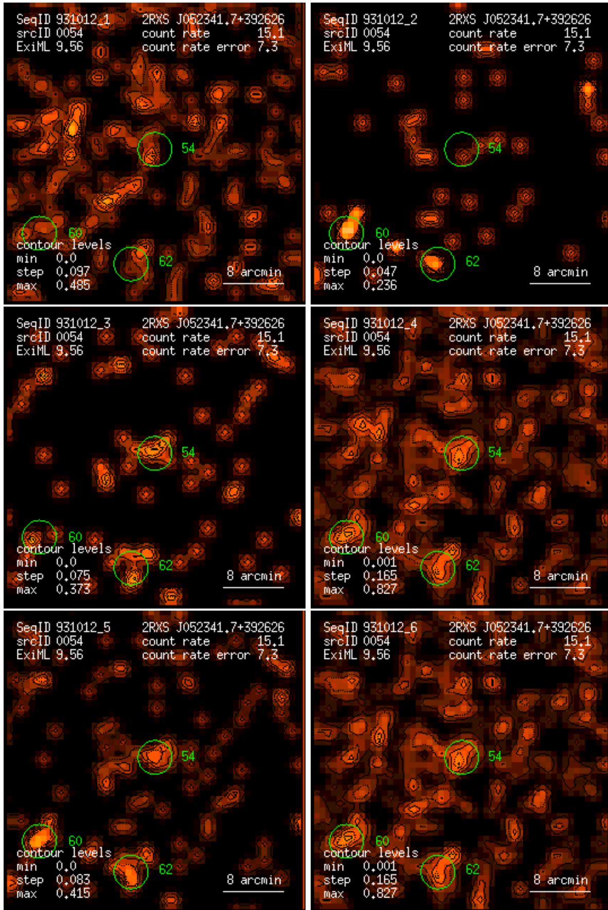
Figure 54: RASS 931012: detection 0054: band rate images, Gaussian filter: (1) PSPC channels 11 – 41, (2) 52 – 90, (3) 91 – 201, (4) 11 – 235, (5) 52 – 201, (6) 11 – 201. Broad band rates in counts/ks. Band rate contour levels in counts/ks/arcmin 2 .
