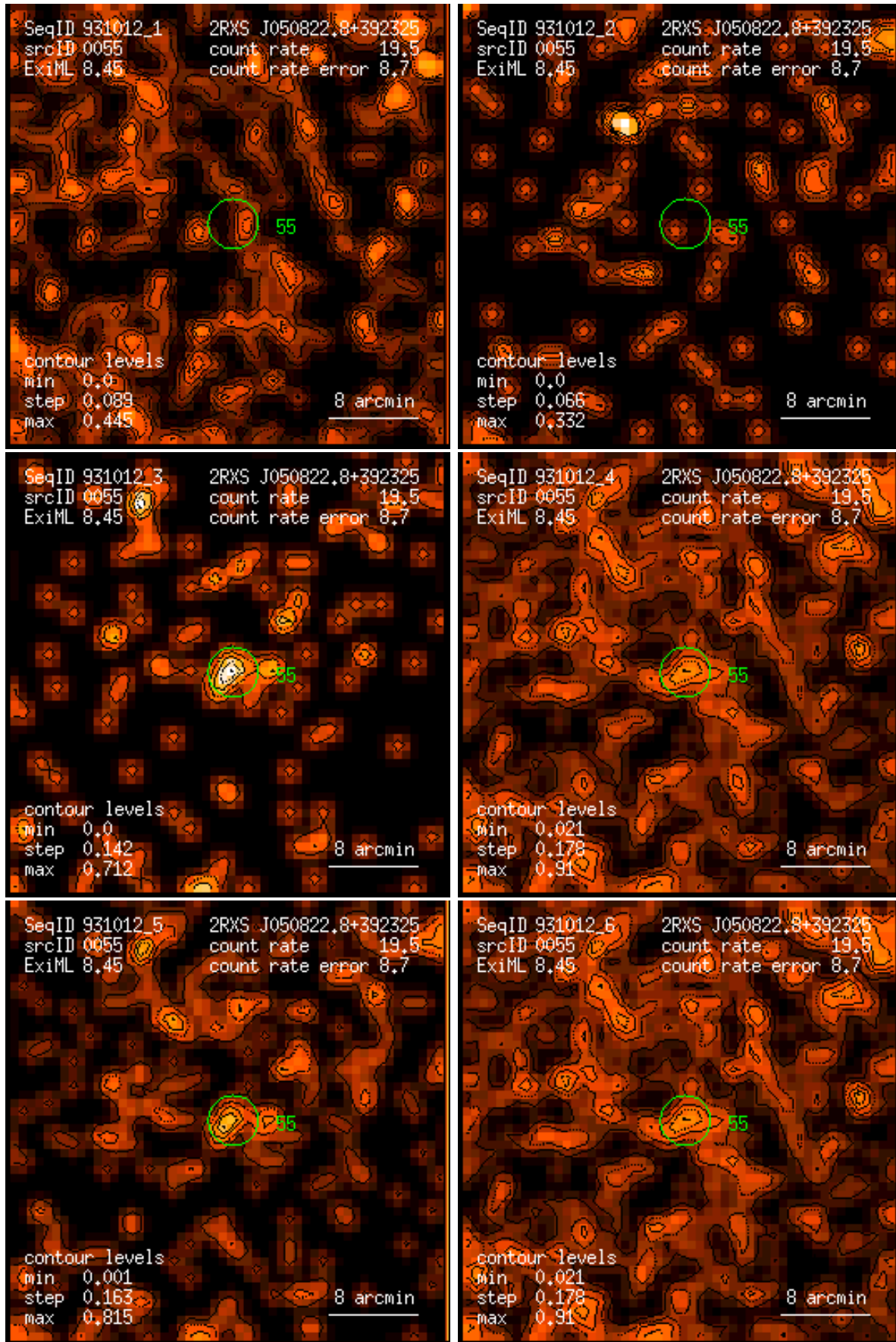
Figure 55: RASS 931012: detection 0055: band rate images, Gaussian filter: (1) PSPC channels 11 – 41, (2) 52 – 90, (3) 91 – 201, (4) 11 – 235, (5) 52 – 201, (6) 11 – 201. Broad band rates in counts/ks. Band rate contour levels in counts/ks/arcmin 2 .
