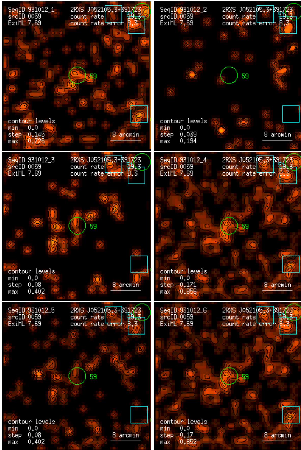
Figure 59: RASS 931012: detection 0059: band rate images, Gaussian filter: (1) PSPC channels 11 – 41, (2) 52 – 90, (3) 91 – 201, (4) 11 – 235, (5) 52 – 201, (6) 11 – 201. Broad band rates in counts/ks. Band rate contour levels in counts/ks/arcmin 2 .
