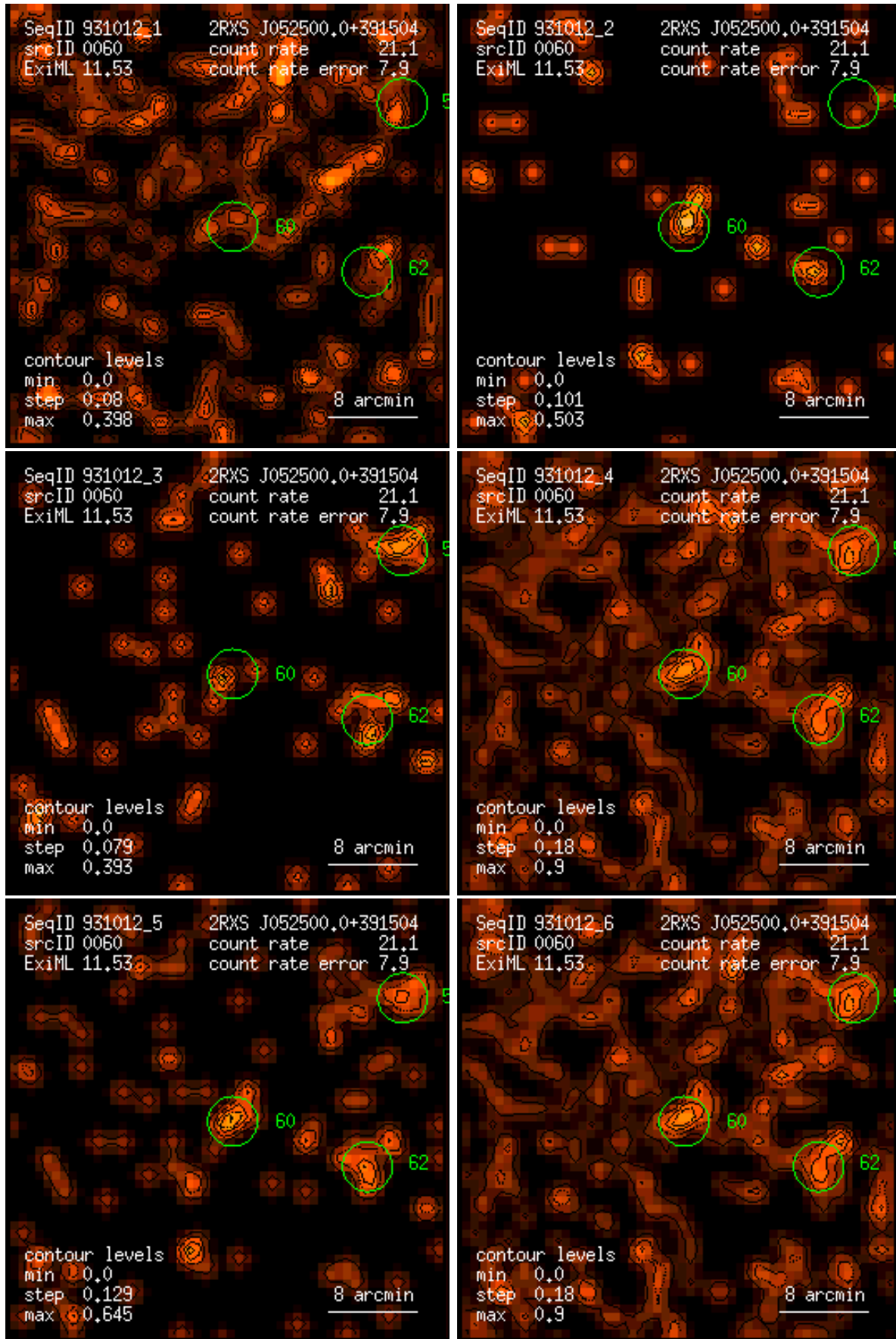
Figure 60: RASS 931012: detection 0060: band rate images, Gaussian filter: (1) PSPC channels 11 – 41, (2) 52 – 90, (3) 91 – 201, (4) 11 – 235, (5) 52 – 201, (6) 11 – 201. Broad band rates in counts/ks. Band rate contour levels in counts/ks/arcmin 2 .
