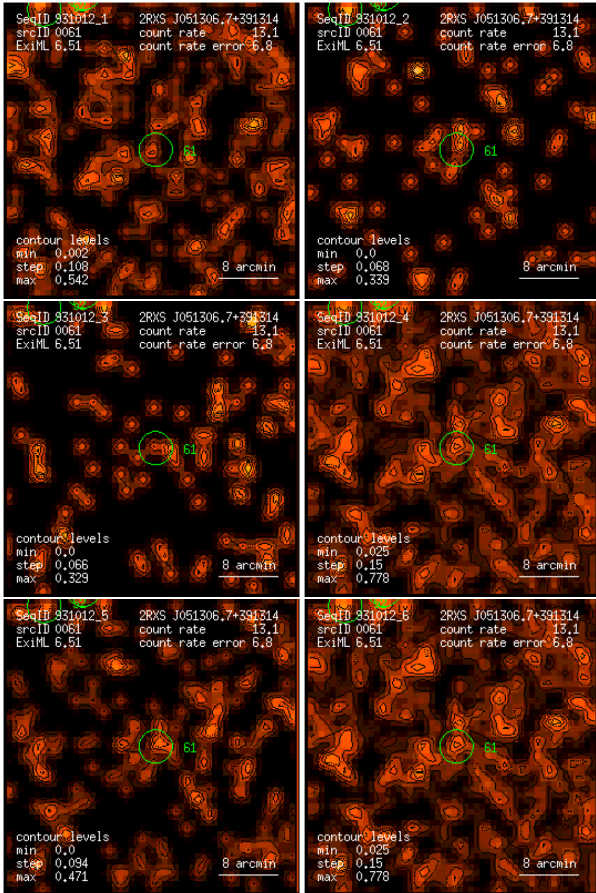
Figure 61: RASS 931012: detection 0061: band rate images, Gaussian filter: (1) PSPC channels 11 – 41, (2) 52 – 90, (3) 91 – 201, (4) 11 – 235, (5) 52 – 201, (6) 11 – 201. Broad band rates in counts/ks. Band rate contour levels in counts/ks/arcmin 2 .
