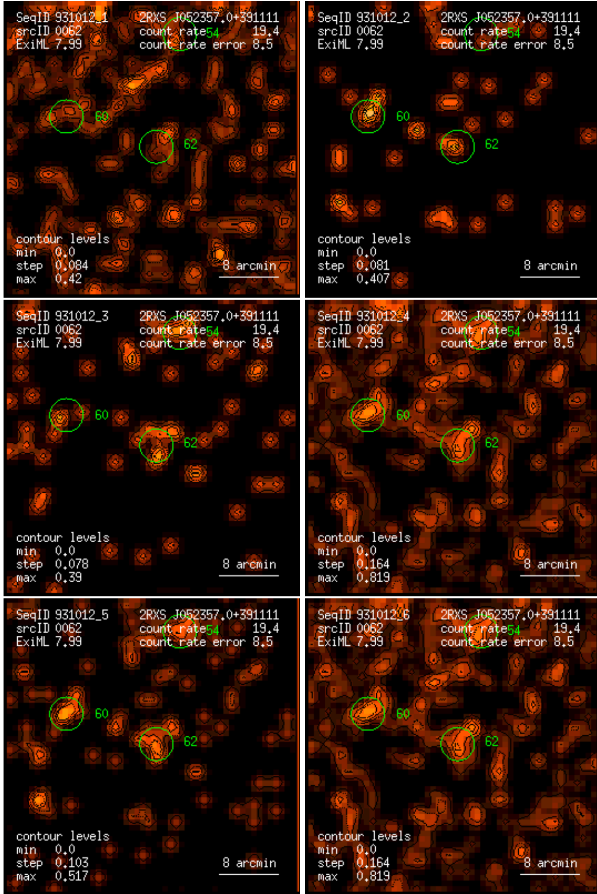
Figure 62: RASS 931012: detection 0062: band rate images, Gaussian filter: (1) PSPC channels 11 – 41, (2) 52 – 90, (3) 91 – 201, (4) 11 – 235, (5) 52 – 201, (6) 11 – 201. Broad band rates in counts/ks. Band rate contour levels in counts/ks/arcmin 2 .
