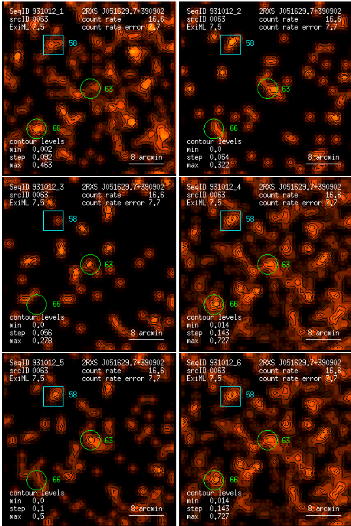
Figure 63: RASS 931012: detection 0063: band rate images, Gaussian filter: (1) PSPC channels 11 – 41, (2) 52 – 90, (3) 91 – 201, (4) 11 – 235, (5) 52 – 201, (6) 11 – 201. Broad band rates in counts/ks. Band rate contour levels in counts/ks/arcmin 2 .
