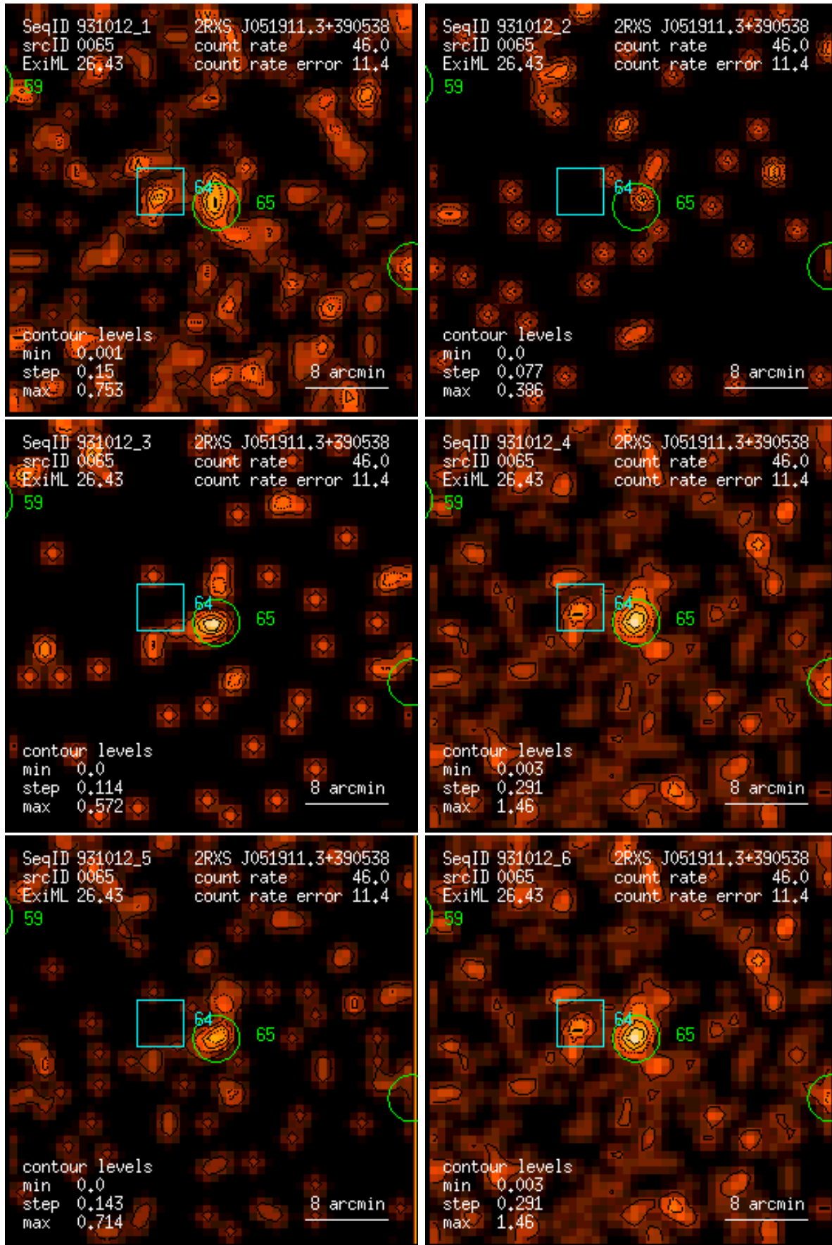
Figure 65: RASS 931012: detection 0065: band rate images, Gaussian filter: (1) PSPC channels 11 – 41, (2) 52 – 90, (3) 91 – 201, (4) 11 – 235, (5) 52 – 201, (6) 11 – 201. Broad band rates in counts/ks. Band rate contour levels in counts/ks/arcmin 2 .
