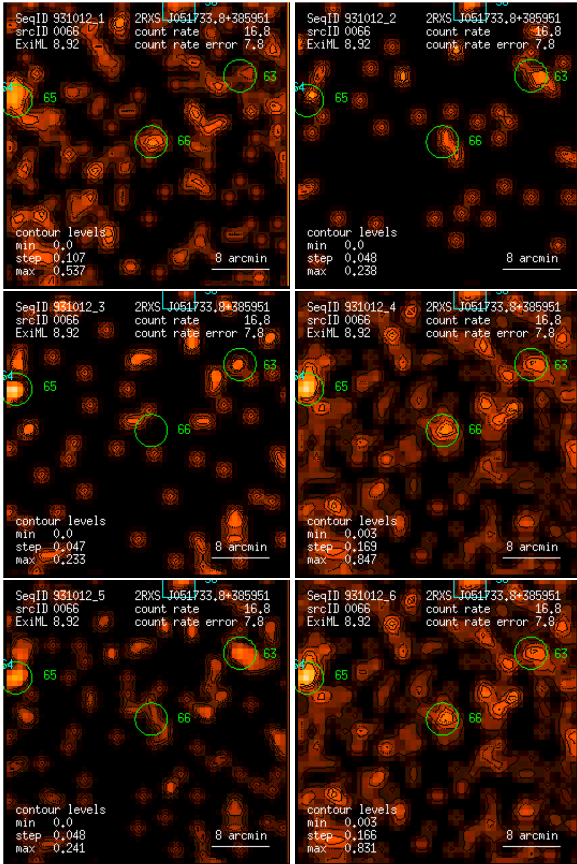
Figure 66: RASS 931012: detection 0066: band rate images, Gaussian filter: (1) PSPC channels 11 – 41, (2) 52 – 90, (3) 91 – 201, (4) 11 – 235, (5) 52 – 201, (6) 11 – 201. Broad band rates in counts/ks. Band rate contour levels in counts/ks/arcmin 2 .
