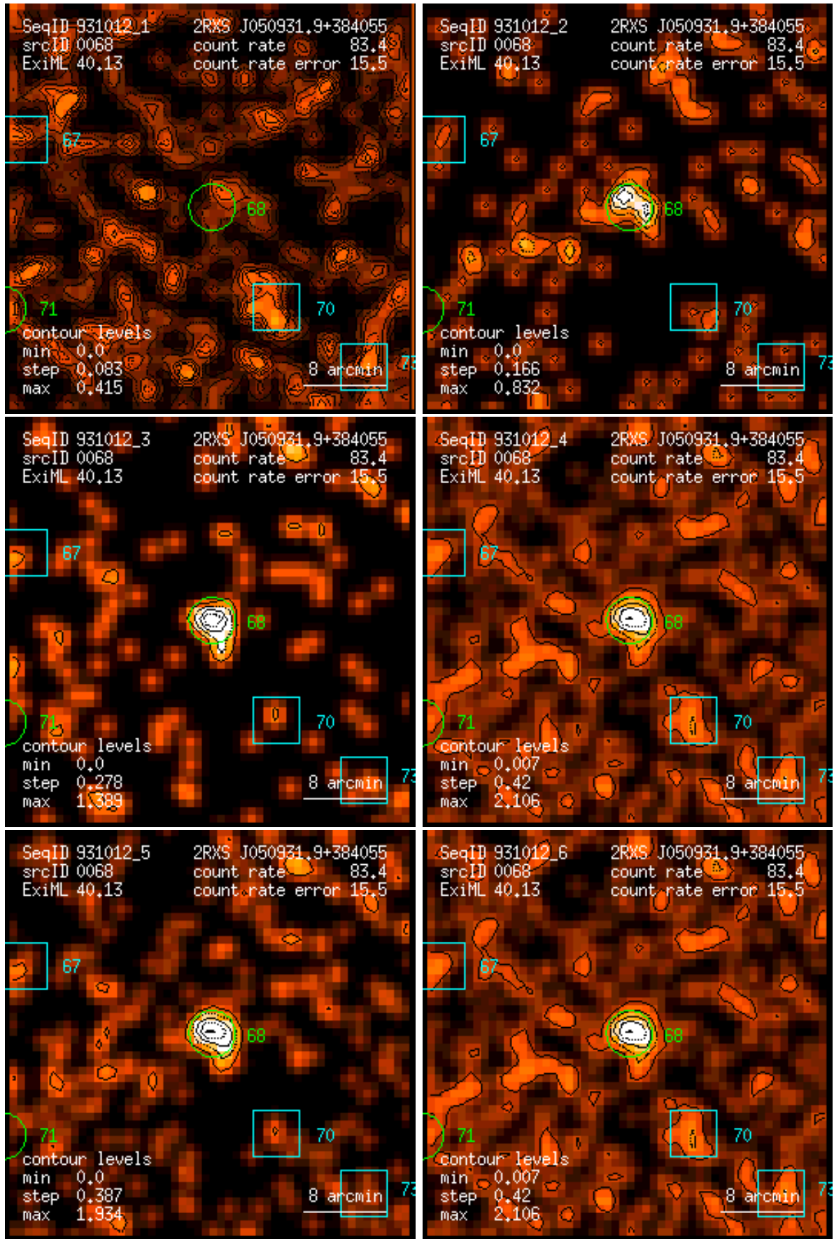
Figure 68: RASS 931012: detection 0068: band rate images, Gaussian filter: (1) PSPC channels 11 – 41, (2) 52 – 90, (3) 91 – 201, (4) 11 – 235, (5) 52 – 201, (6) 11 – 201. Broad band rates in counts/ks. Band rate contour levels in counts/ks/arcmin 2 .
