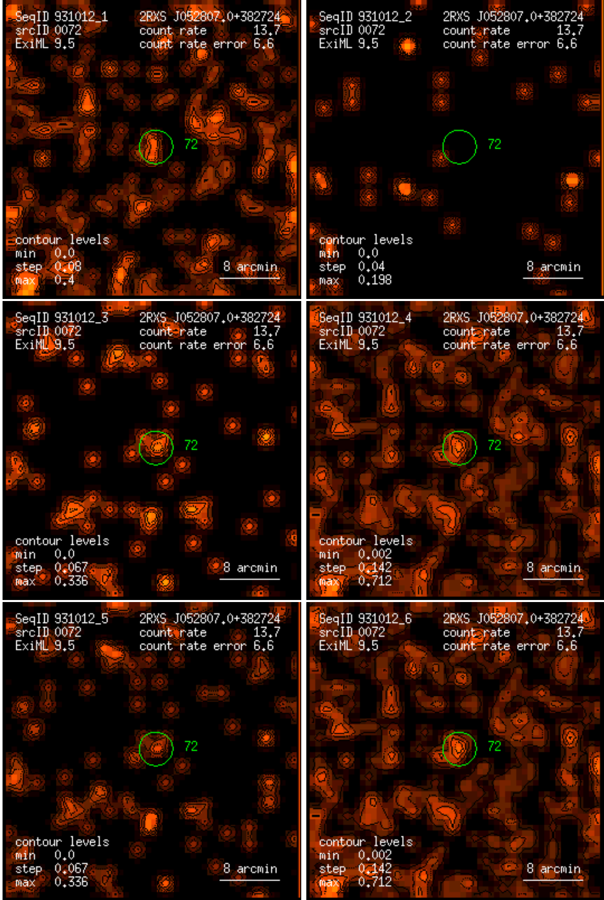
Figure 72: RASS 931012: detection 0072: band rate images, Gaussian filter: (1) PSPC channels 11 – 41, (2) 52 – 90, (3) 91 – 201, (4) 11 – 235, (5) 52 – 201, (6) 11 – 201. Broad band rates in counts/ks. Band rate contour levels in counts/ks/arcmin 2 .
