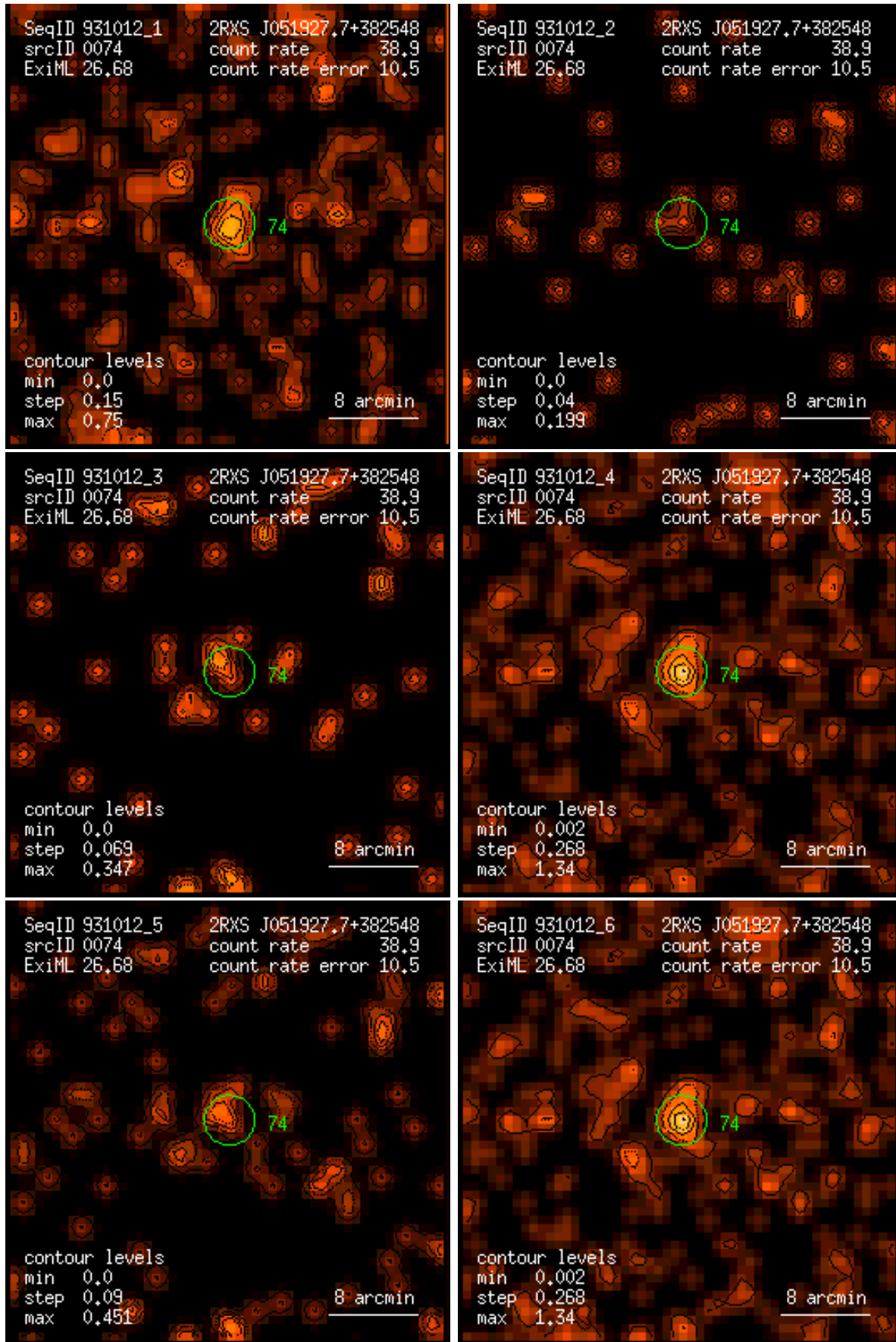
Figure 74: RASS 931012: detection 0074: band rate images, Gaussian filter: (1) PSPC channels 11 – 41, (2) 52 – 90, (3) 91 – 201, (4) 11 – 235, (5) 52 – 201, (6) 11 – 201. Broad band rates in counts/ks. Band rate contour levels in counts/ks/arcmin 2 .
