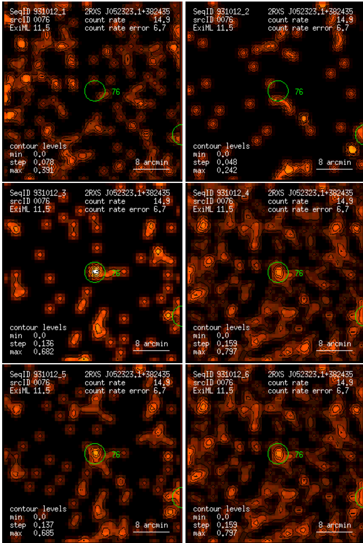
Figure 76: RASS 931012: detection 0076: band rate images, Gaussian filter: (1) PSPC channels 11 – 41, (2) 52 – 90, (3) 91 – 201, (4) 11 – 235, (5) 52 – 201, (6) 11 – 201. Broad band rates in counts/ks. Band rate contour levels in counts/ks/arcmin 2 .
