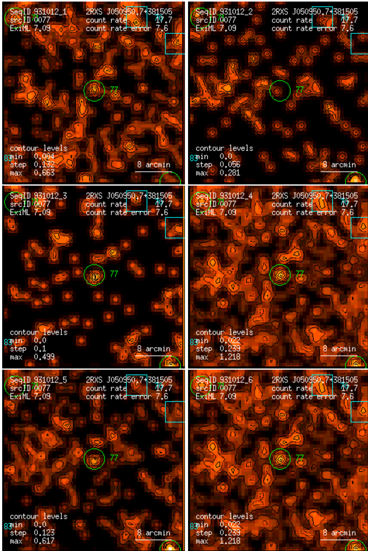
Figure 77: RASS 931012: detection 0077: band rate images, Gaussian filter: (1) PSPC channels 11 – 41, (2) 52 – 90, (3) 91 – 201, (4) 11 – 235, (5) 52 – 201, (6) 11 – 201. Broad band rates in counts/ks. Band rate contour levels in counts/ks/arcmin 2 .
