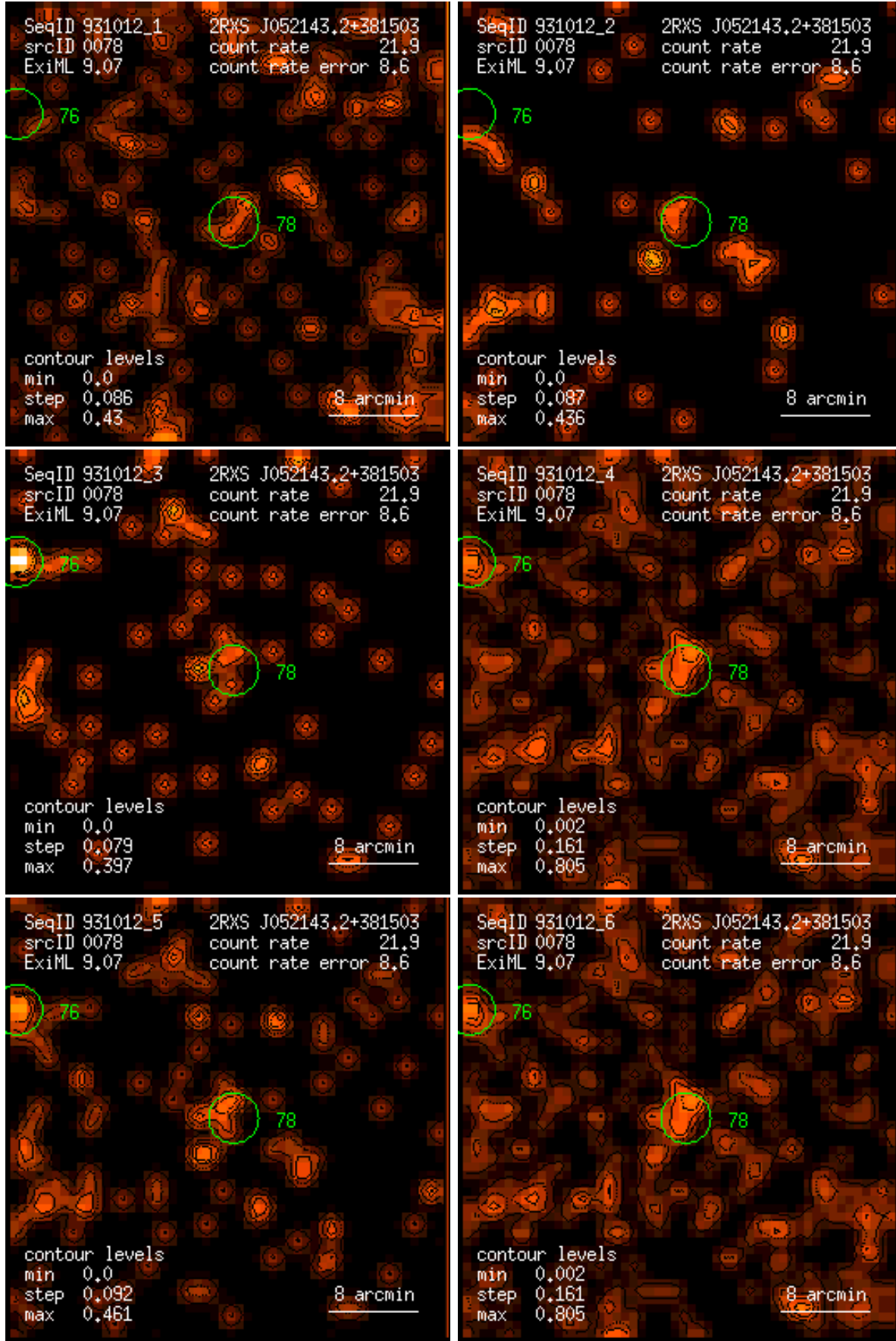
Figure 78: RASS 931012: detection 0078: band rate images, Gaussian filter: (1) PSPC channels 11 – 41, (2) 52 – 90, (3) 91 – 201, (4) 11 – 235, (5) 52 – 201, (6) 11 – 201. Broad band rates in counts/ks. Band rate contour levels in counts/ks/arcmin 2 .
