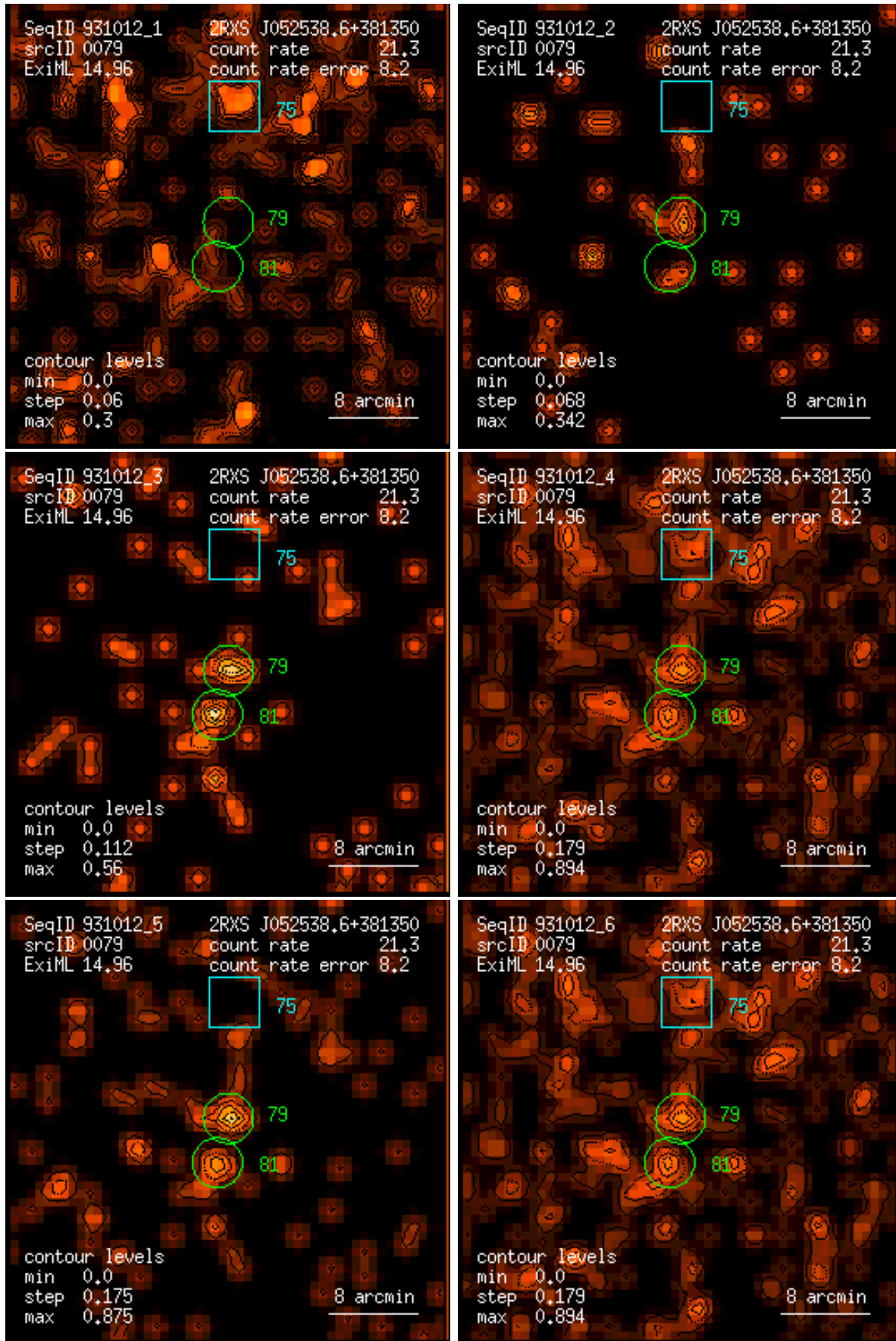
Figure 79: RASS 931012: detection 0079: band rate images, Gaussian filter: (1) PSPC channels 11 – 41, (2) 52 – 90, (3) 91 – 201, (4) 11 – 235, (5) 52 – 201, (6) 11 – 201. Broad band rates in counts/ks. Band rate contour levels in counts/ks/arcmin 2 .
