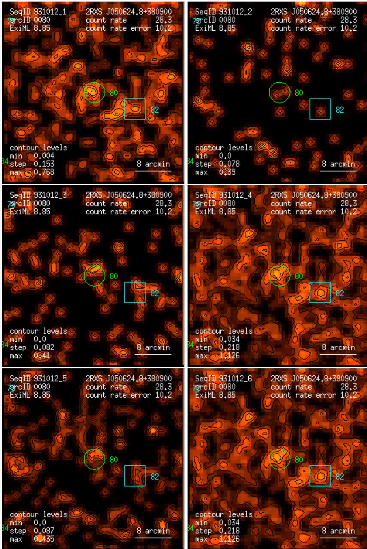
Figure 80: RASS 931012: detection 0080: band rate images, Gaussian filter: (1) PSPC channels 11 – 41, (2) 52 – 90, (3) 91 – 201, (4) 11 – 235, (5) 52 – 201, (6) 11 – 201. Broad band rates in counts/ks. Band rate contour levels in counts/ks/arcmin 2 .
