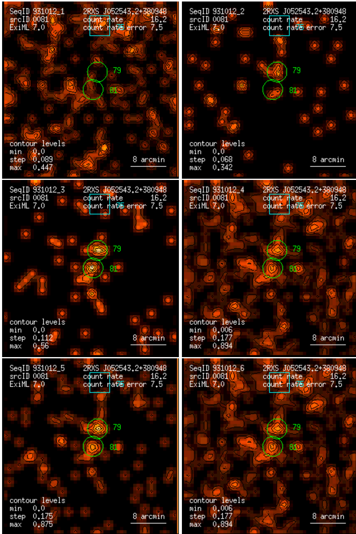
Figure 81: RASS 931012: detection 0081: band rate images, Gaussian filter: (1) PSPC channels 11 – 41, (2) 52 – 90, (3) 91 – 201, (4) 11 – 235, (5) 52 – 201, (6) 11 – 201. Broad band rates in counts/ks. Band rate contour levels in counts/ks/arcmin 2 .
