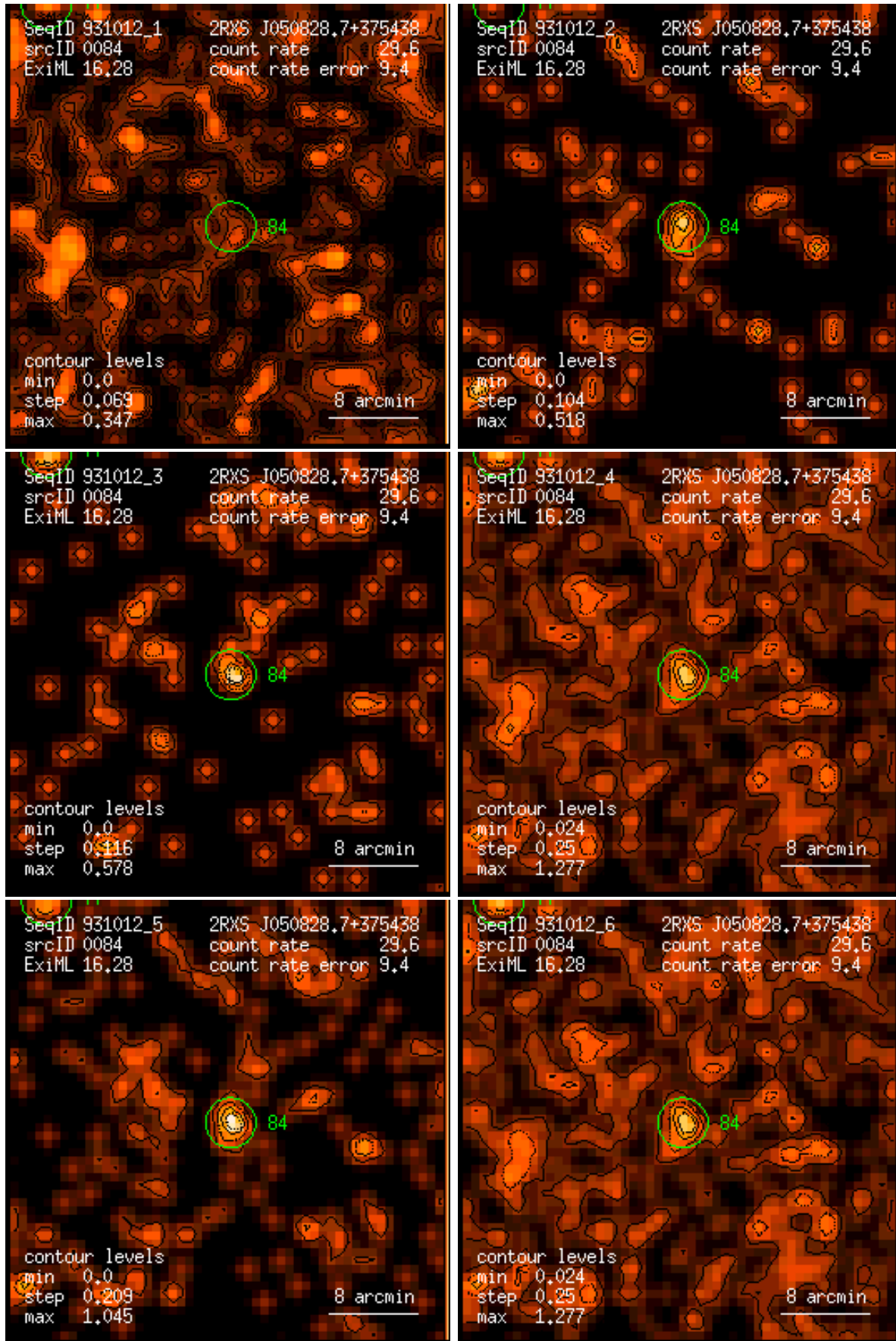
Figure 84: RASS 931012: detection 0084: band rate images, Gaussian filter: (1) PSPC channels 11 – 41, (2) 52 – 90, (3) 91 – 201, (4) 11 – 235, (5) 52 – 201, (6) 11 – 201. Broad band rates in counts/ks. Band rate contour levels in counts/ks/arcmin 2 .
