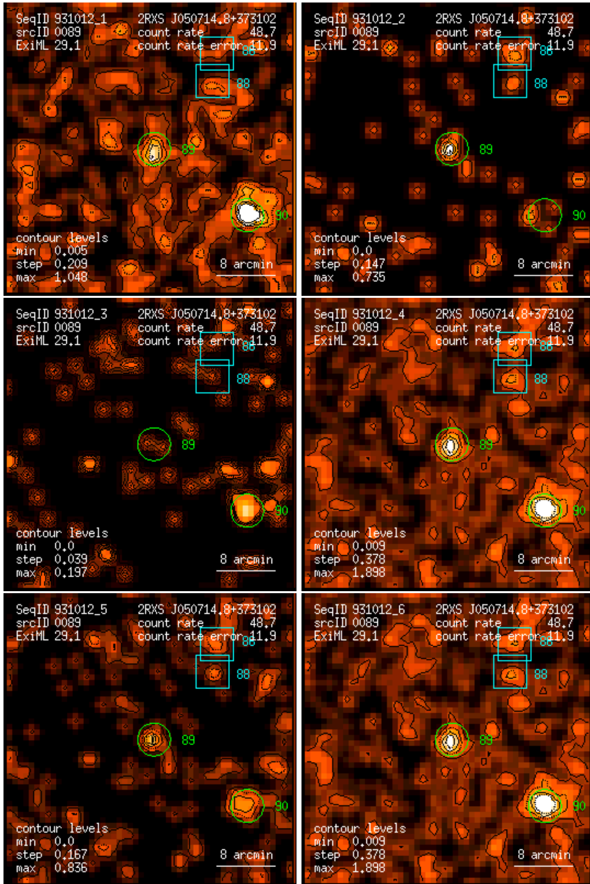
Figure 89: RASS 931012: detection 0089: band rate images, Gaussian filter: (1) PSPC channels 11 – 41, (2) 52 – 90, (3) 91 – 201, (4) 11 – 235, (5) 52 – 201, (6) 11 – 201. Broad band rates in counts/ks. Band rate contour levels in counts/ks/arcmin 2 .
