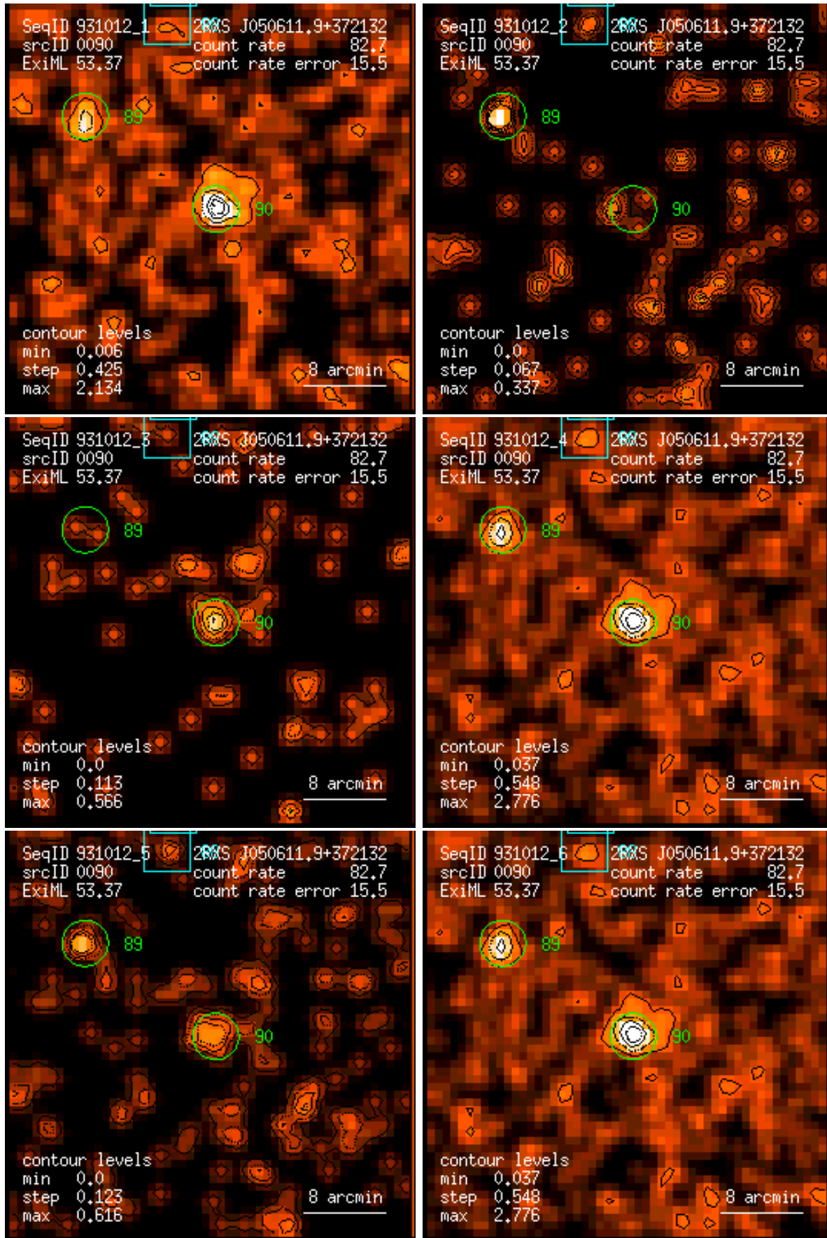
Figure 90: RASS 931012: detection 0090: band rate images, Gaussian filter: (1) PSPC channels 11 – 41, (2) 52 – 90, (3) 91 – 201, (4) 11 – 235, (5) 52 – 201, (6) 11 – 201. Broad band rates in counts/ks. Band rate contour levels in counts/ks/arcmin 2 .
