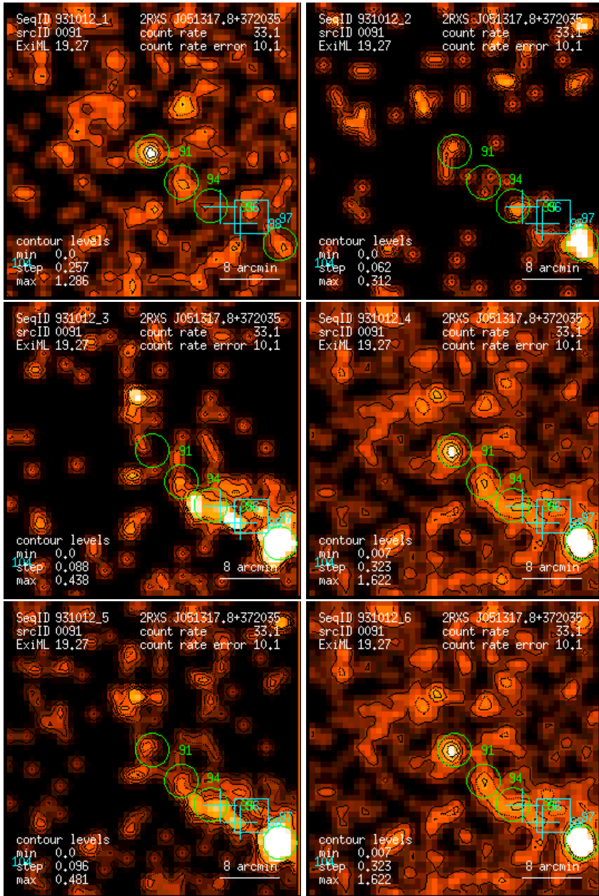
Figure 91: RASS 931012: detection 0091: band rate images, Gaussian filter: (1) PSPC channels 11 – 41, (2) 52 – 90, (3) 91 – 201, (4) 11 – 235, (5) 52 – 201, (6) 11 – 201. Broad band rates in counts/ks. Band rate contour levels in counts/ks/arcmin 2 .
