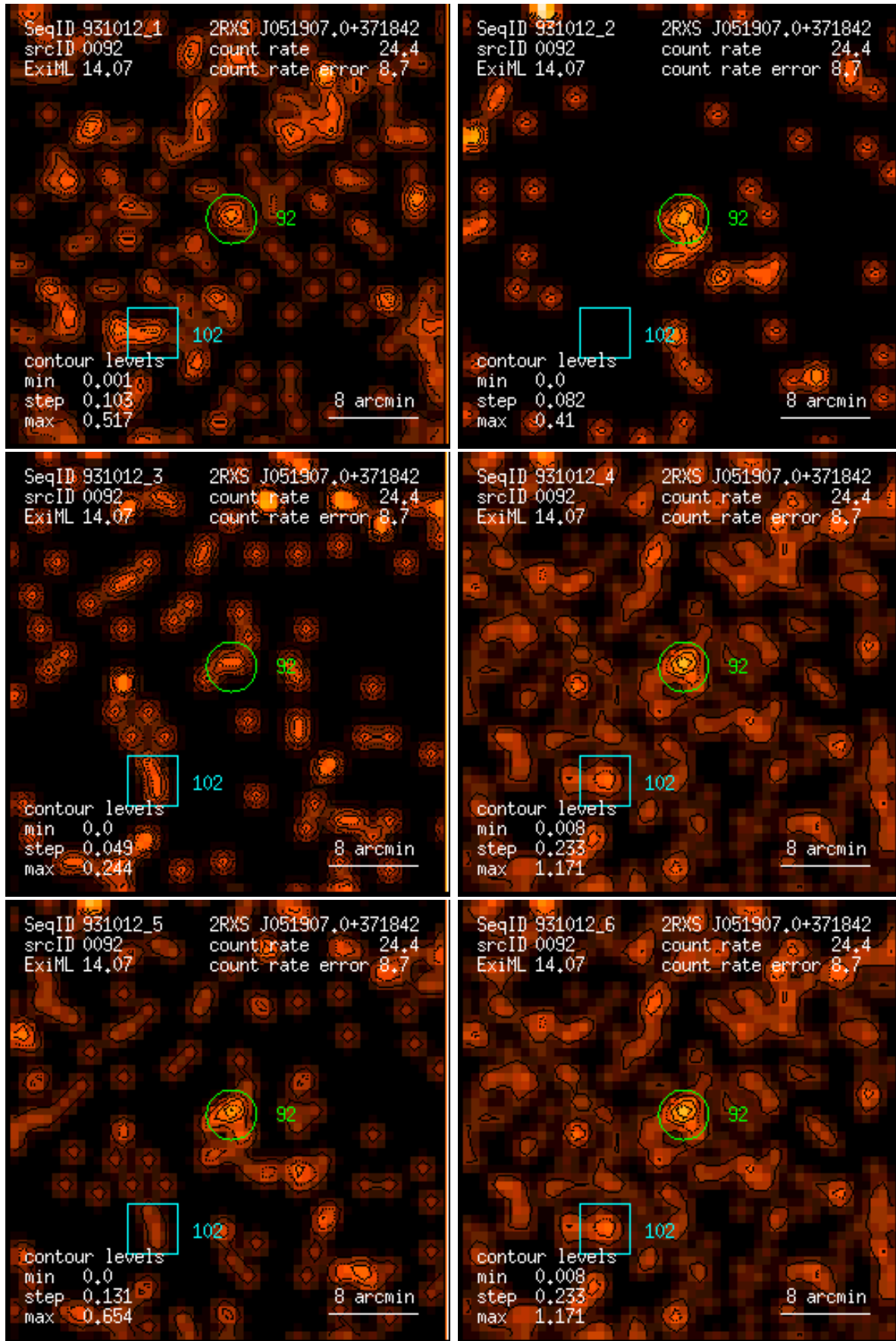
Figure 92: RASS 931012: detection 0092: band rate images, Gaussian filter: (1) PSPC channels 11 – 41, (2) 52 – 90, (3) 91 – 201, (4) 11 – 235, (5) 52 – 201, (6) 11 – 201. Broad band rates in counts/ks. Band rate contour levels in counts/ks/arcmin 2 .
