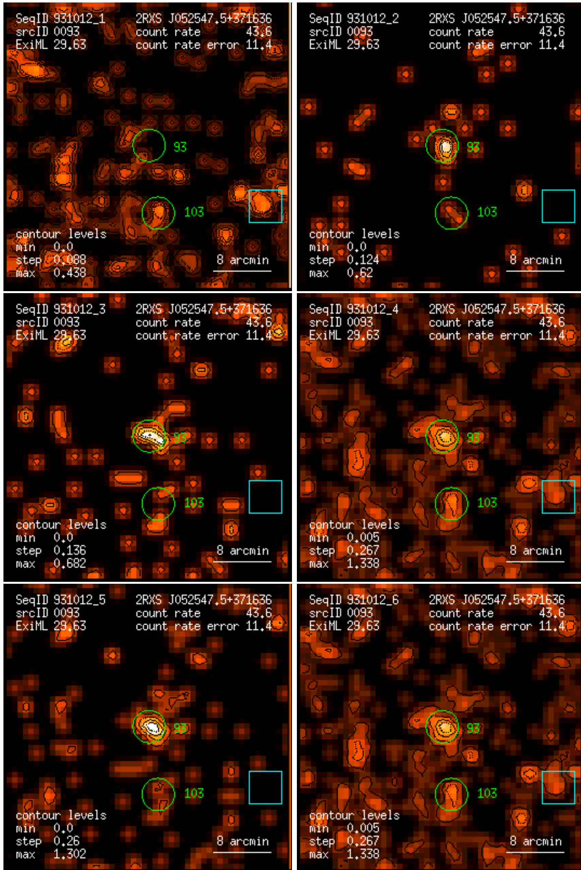
Figure 93: RASS 931012: detection 0093: band rate images, Gaussian filter: (1) PSPC channels 11 – 41, (2) 52 – 90, (3) 91 – 201, (4) 11 – 235, (5) 52 – 201, (6) 11 – 201. Broad band rates in counts/ks. Band rate contour levels in counts/ks/arcmin 2 .
