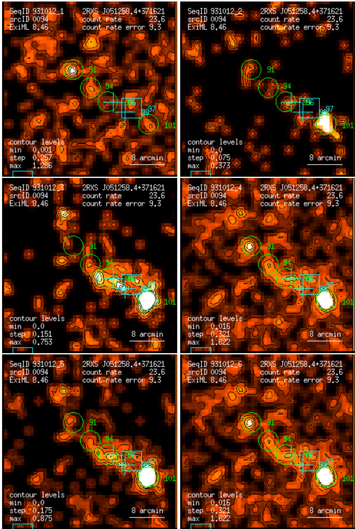
Figure 94: RASS 931012: detection 0094: band rate images, Gaussian filter: (1) PSPC channels 11 – 41, (2) 52 – 90, (3) 91 – 201, (4) 11 – 235, (5) 52 – 201, (6) 11 – 201. Broad band rates in counts/ks. Band rate contour levels in counts/ks/arcmin 2 .
