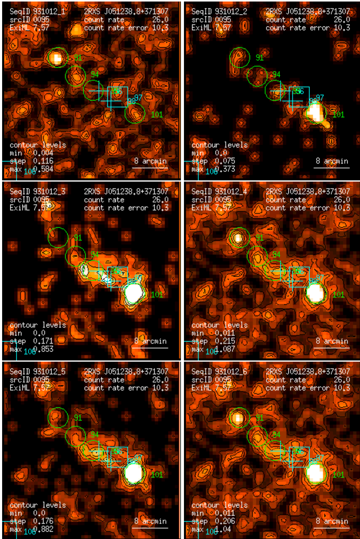
Figure 95: RASS 931012: detection 0095: band rate images, Gaussian filter: (1) PSPC channels 11 – 41, (2) 52 – 90, (3) 91 – 201, (4) 11 – 235, (5) 52 – 201, (6) 11 – 201. Broad band rates in counts/ks. Band rate contour levels in counts/ks/arcmin 2 .
