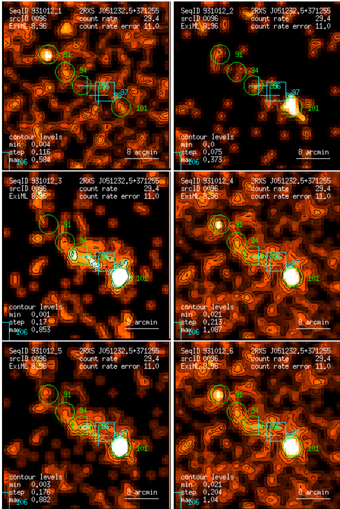
Figure 96: RASS 931012: detection 0096: band rate images, Gaussian filter: (1) PSPC channels 11 – 41, (2) 52 – 90, (3) 91 – 201, (4) 11 – 235, (5) 52 – 201, (6) 11 – 201. Broad band rates in counts/ks. Band rate contour levels in counts/ks/arcmin 2 .
