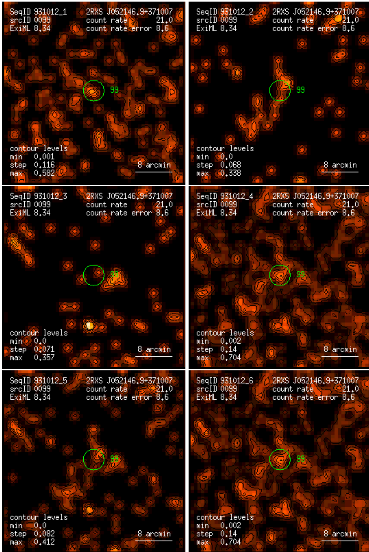
Figure 99: RASS 931012: detection 0099: band rate images, Gaussian filter: (1) PSPC channels 11 – 41, (2) 52 – 90, (3) 91 – 201, (4) 11 – 235, (5) 52 – 201, (6) 11 – 201. Broad band rates in counts/ks. Band rate contour levels in counts/ks/arcmin 2 .
