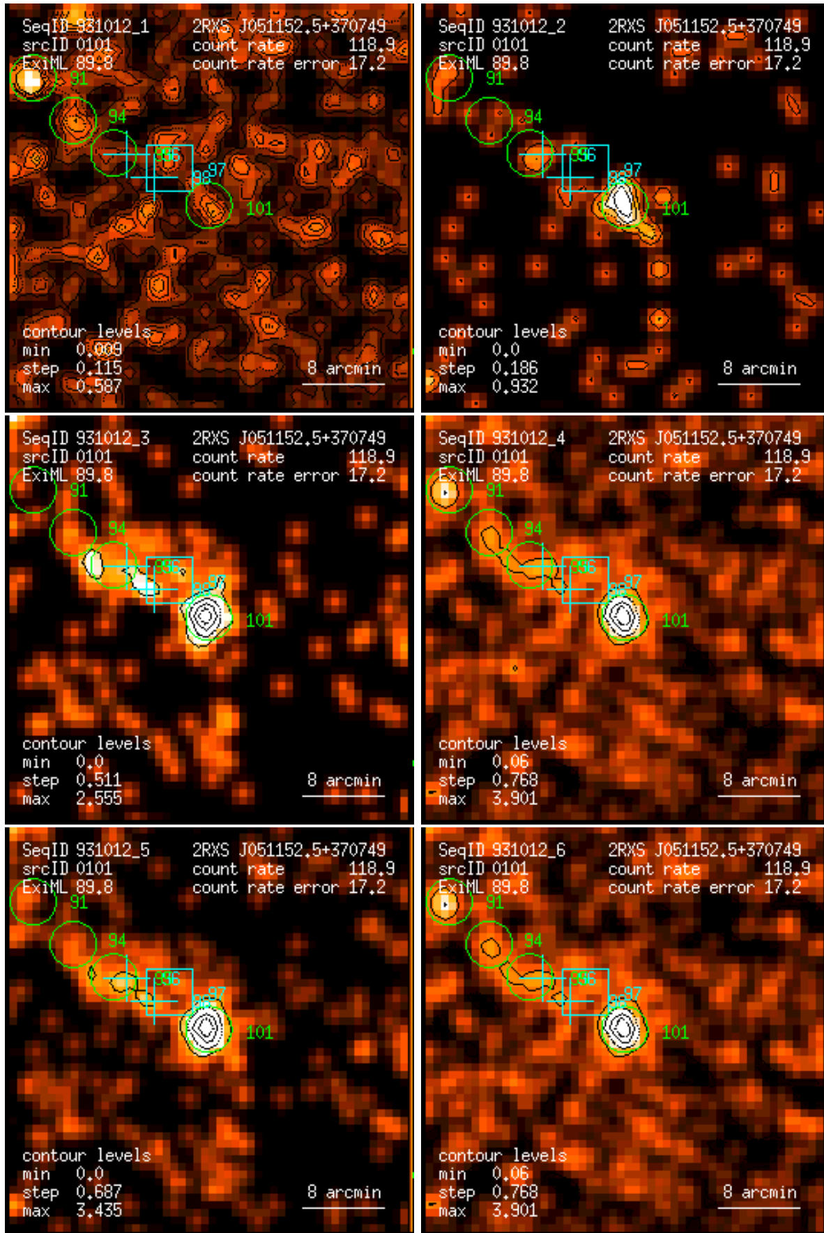
Figure 101: RASS 931012: detection 0101: band rate images, Gaussian filter: (1) PSPC channels 11 – 41, (2) 52 – 90, (3) 91 – 201, (4) 11 – 235, (5) 52 – 201, (6) 11 – 201. Broad band rates in counts/ks. Band rate contour levels in counts/ks/arcmin 2 .
