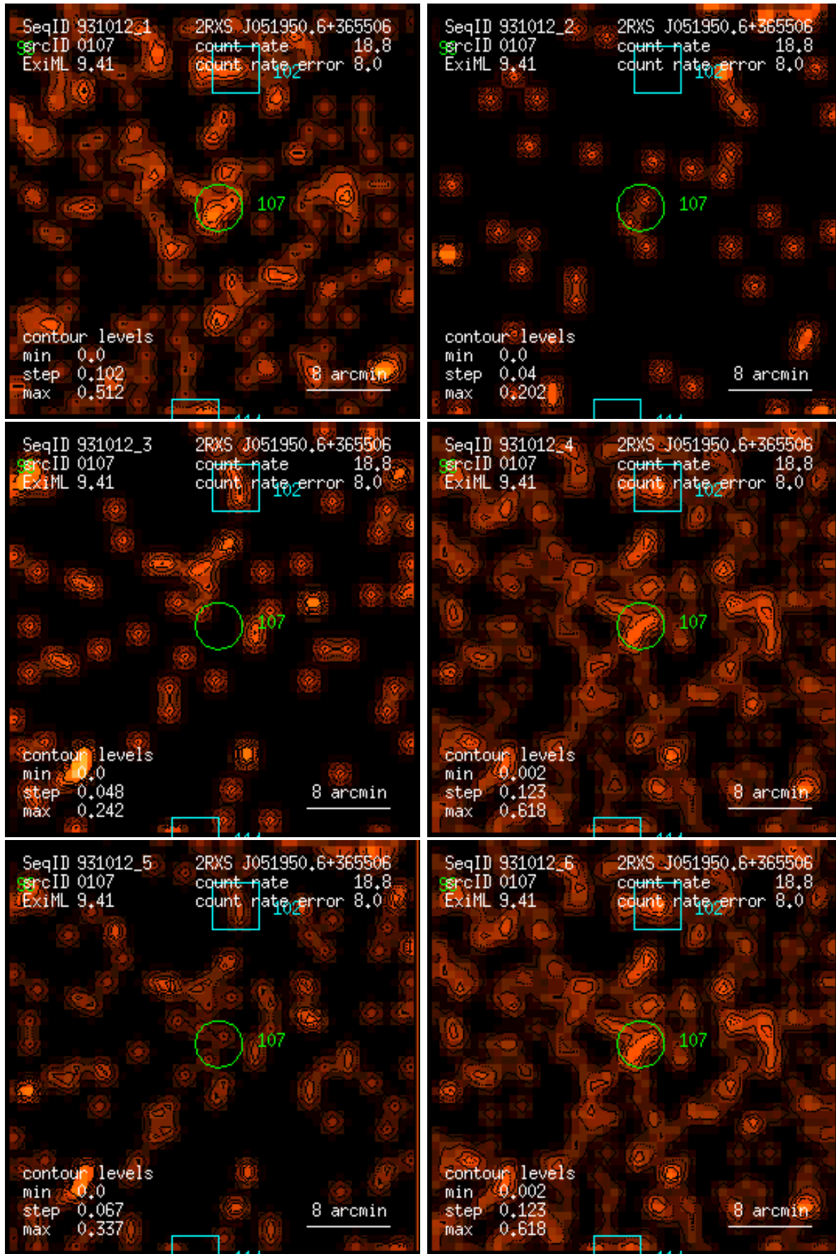
Figure 107: RASS 931012: detection 0107: band rate images, Gaussian filter: (1) PSPC channels 11 – 41, (2) 52 – 90, (3) 91 – 201, (4) 11 – 235, (5) 52 – 201, (6) 11 – 201. Broad band rates in counts/ks. Band rate contour levels in counts/ks/arcmin 2 .
