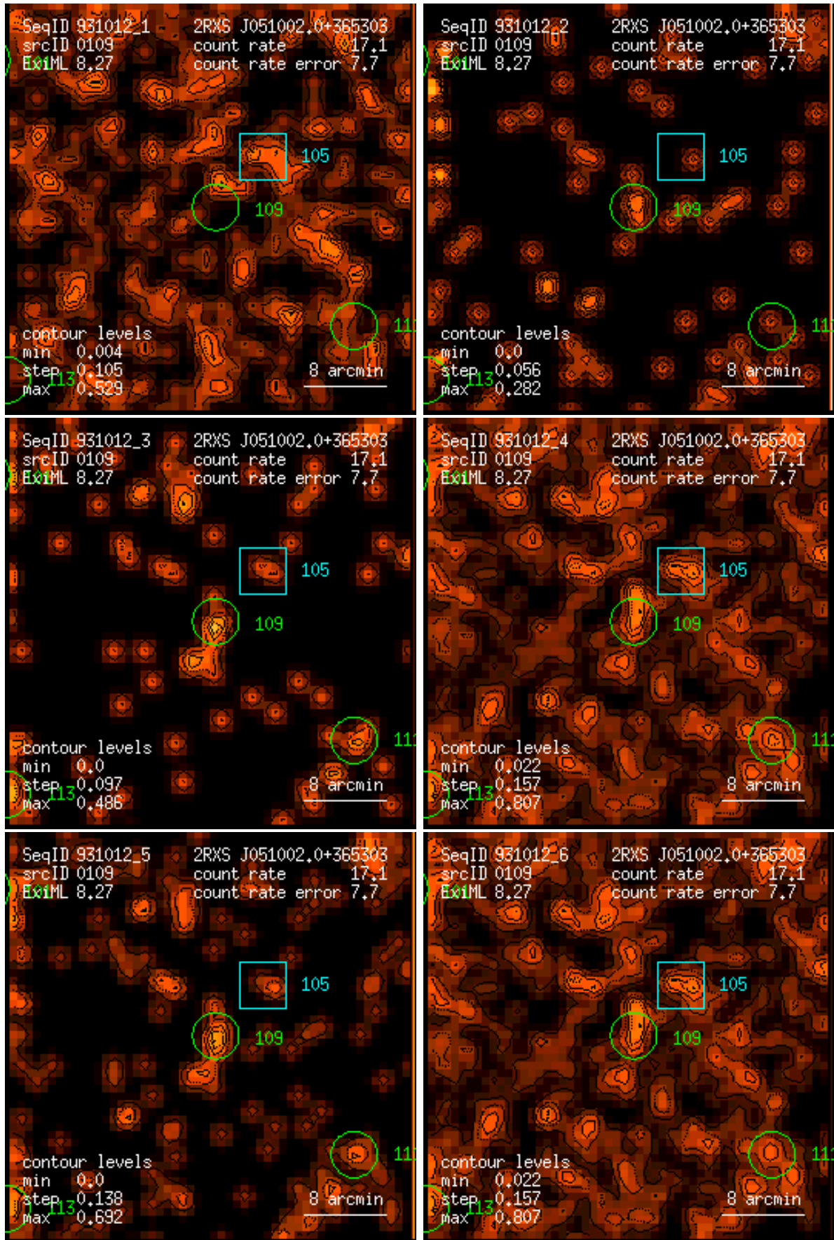
Figure 109: RASS 931012: detection 0109: band rate images, Gaussian filter: (1) PSPC channels 11 – 41, (2) 52 – 90, (3) 91 – 201, (4) 11 – 235, (5) 52 – 201, (6) 11 – 201. Broad band rates in counts/ks. Band rate contour levels in counts/ks/arcmin 2 .
