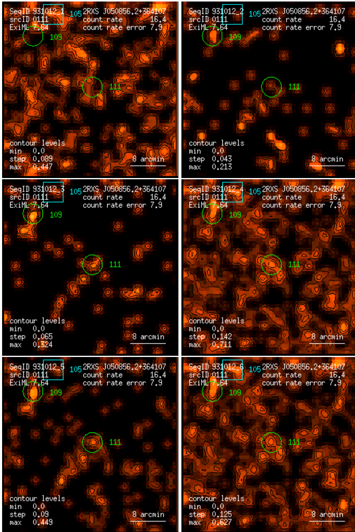
Figure 111: RASS 931012: detection 0111: band rate images, Gaussian filter: (1) PSPC channels 11 – 41, (2) 52 – 90, (3) 91 – 201, (4) 11 – 235, (5) 52 – 201, (6) 11 – 201. Broad band rates in counts/ks. Band rate contour levels in counts/ks/arcmin 2 .
