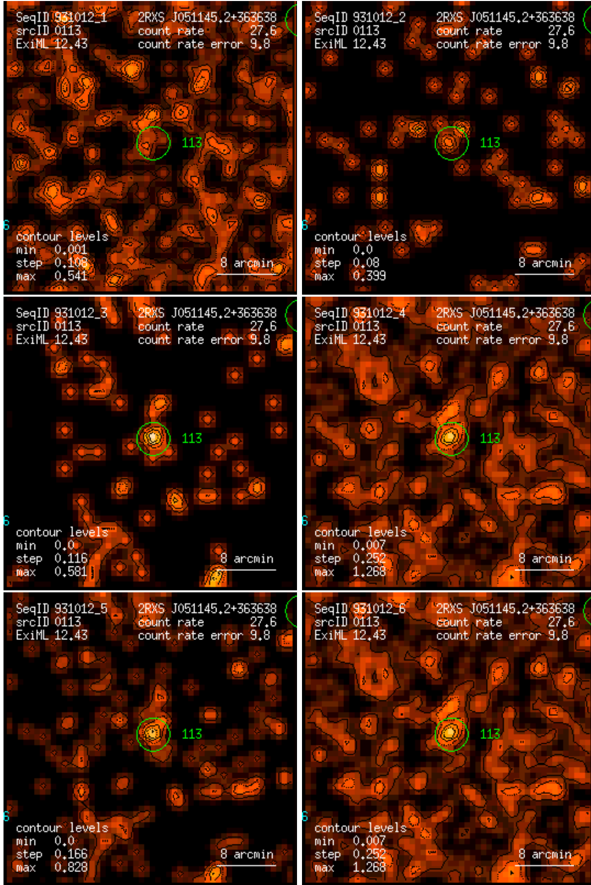
Figure 113: RASS 931012: detection 0113: band rate images, Gaussian filter: (1) PSPC channels 11 – 41, (2) 52 – 90, (3) 91 – 201, (4) 11 – 235, (5) 52 – 201, (6) 11 – 201. Broad band rates in counts/ks. Band rate contour levels in counts/ks/arcmin 2 .
