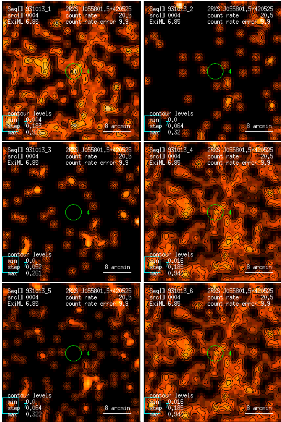
Figure 4: RASS 931013: detection 0004: band rate images, Gaussian filter: (1) PSPC channels 11 – 41, (2) 52 – 90, (3) 91 – 201, (4) 11 – 235, (5) 52 – 201, (6) 11 – 201. Broad band rates in counts/ks. Band rate contour levels in counts/ks/arcmin 2 .
