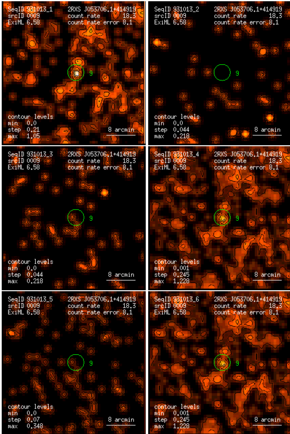
Figure 9: RASS 931013: detection 0009: band rate images, Gaussian filter: (1) PSPC channels 11 – 41, (2) 52 – 90, (3) 91 – 201, (4) 11 – 235, (5) 52 – 201, (6) 11 – 201. Broad band rates in counts/ks. Band rate contour levels in counts/ks/arcmin 2 .
