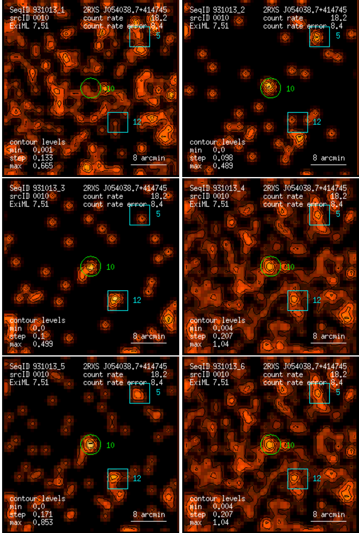
Figure 10: RASS 931013: detection 0010: band rate images, Gaussian filter: (1) PSPC channels 11 – 41, (2) 52 – 90, (3) 91 – 201, (4) 11 – 235, (5) 52 – 201, (6) 11 – 201. Broad band rates in counts/ks. Band rate contour levels in counts/ks/arcmin 2 .
