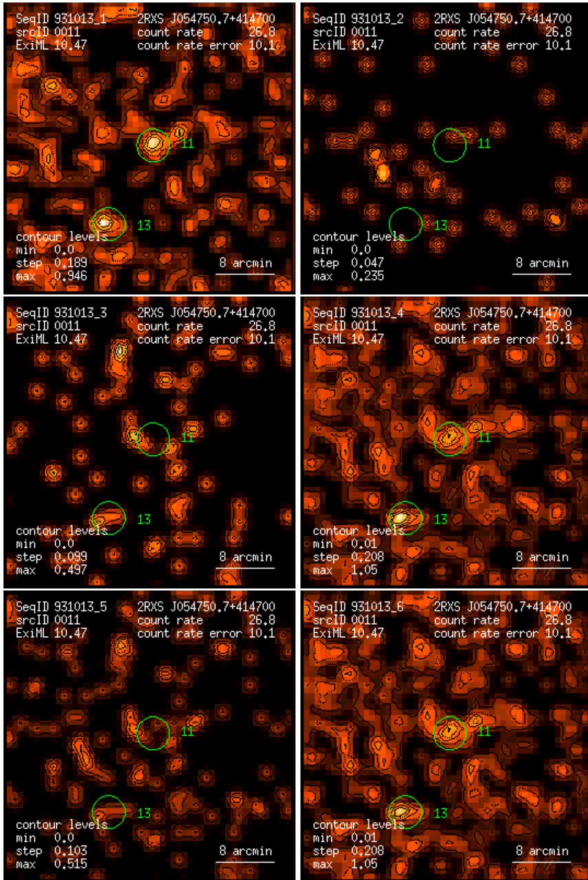
Figure 11: RASS 931013: detection 0011: band rate images, Gaussian filter: (1) PSPC channels 11 – 41, (2) 52 – 90, (3) 91 – 201, (4) 11 – 235, (5) 52 – 201, (6) 11 – 201. Broad band rates in counts/ks. Band rate contour levels in counts/ks/arcmin 2 .
