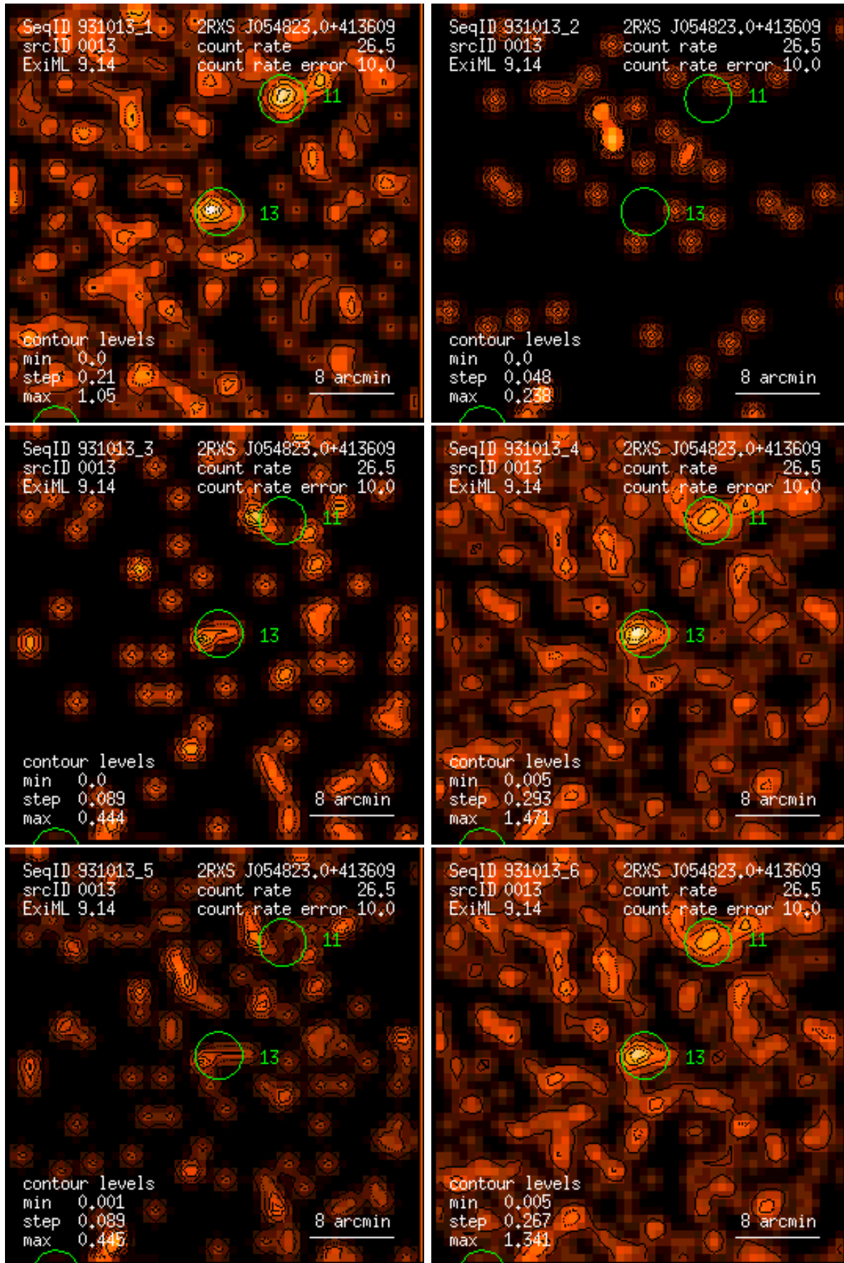
Figure 13: RASS 931013: detection 0013: band rate images, Gaussian filter: (1) PSPC channels 11 – 41, (2) 52 – 90, (3) 91 – 201, (4) 11 – 235, (5) 52 – 201, (6) 11 – 201. Broad band rates in counts/ks. Band rate contour levels in counts/ks/arcmin 2 .
