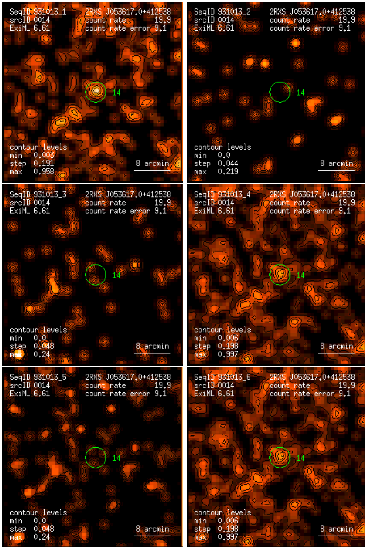
Figure 14: RASS 931013: detection 0014: band rate images, Gaussian filter: (1) PSPC channels 11 – 41, (2) 52 – 90, (3) 91 – 201, (4) 11 – 235, (5) 52 – 201, (6) 11 – 201. Broad band rates in counts/ks. Band rate contour levels in counts/ks/arcmin 2 .
