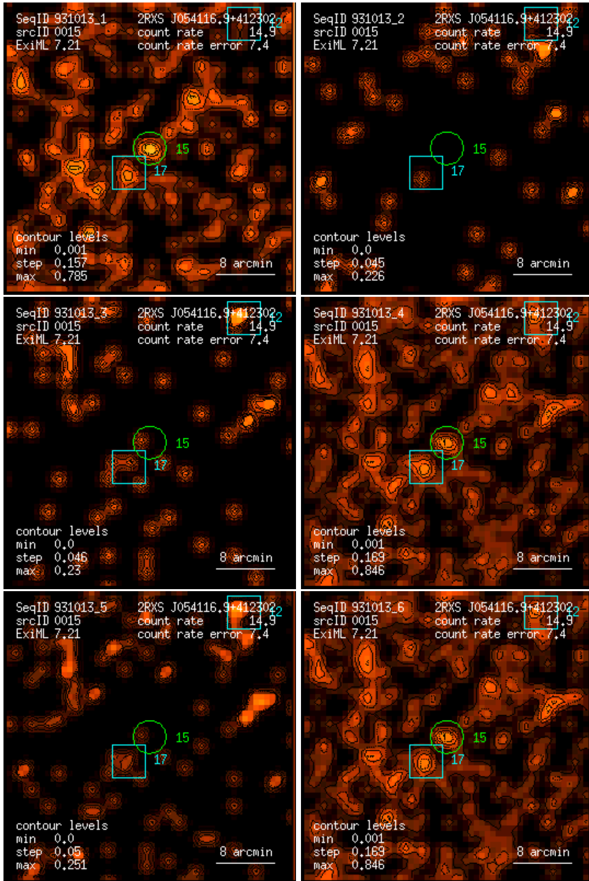
Figure 15: RASS 931013: detection 0015: band rate images, Gaussian filter: (1) PSPC channels 11 – 41, (2) 52 – 90, (3) 91 – 201, (4) 11 – 235, (5) 52 – 201, (6) 11 – 201. Broad band rates in counts/ks. Band rate contour levels in counts/ks/arcmin 2 .
