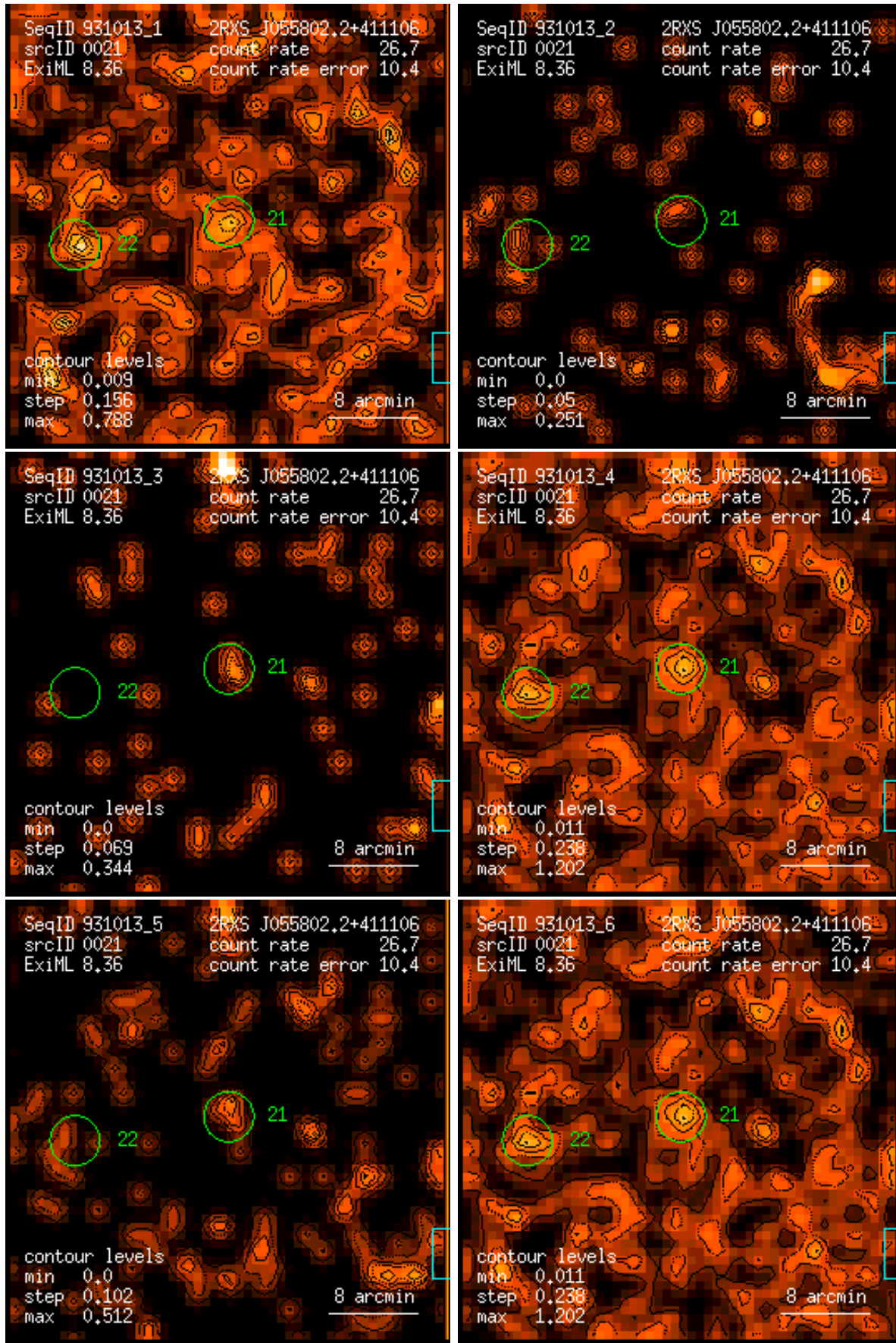
Figure 21: RASS 931013: detection 0021: band rate images, Gaussian filter: (1) PSPC channels 11 – 41, (2) 52 – 90, (3) 91 – 201, (4) 11 – 235, (5) 52 – 201, (6) 11 – 201. Broad band rates in counts/ks. Band rate contour levels in counts/ks/arcmin 2 .
